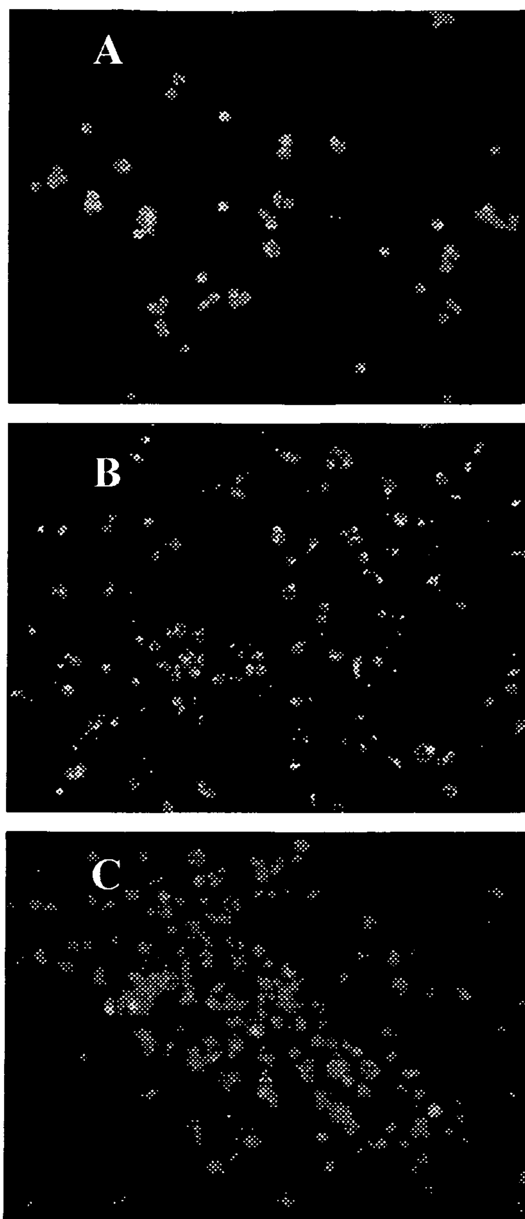
5 Figure 10: Induction of apoptosis in MCF-7 cells by new pyrazolo[4,3-d]pyrimidine 12. A MCF-7, apoptotic cells: 6 h, 12, 20 \mu M, B MCF-7, secondarily necrotic cell (i.e. necrotic following apoptosis), 12 h, 12, 40 \mu M; C MCF-7, necrotic cells, 24h, 12, 40 \mu M. Annexin FITC V (Mol. Probes) and propidium iodide labelling: annexin – green, PI – red
