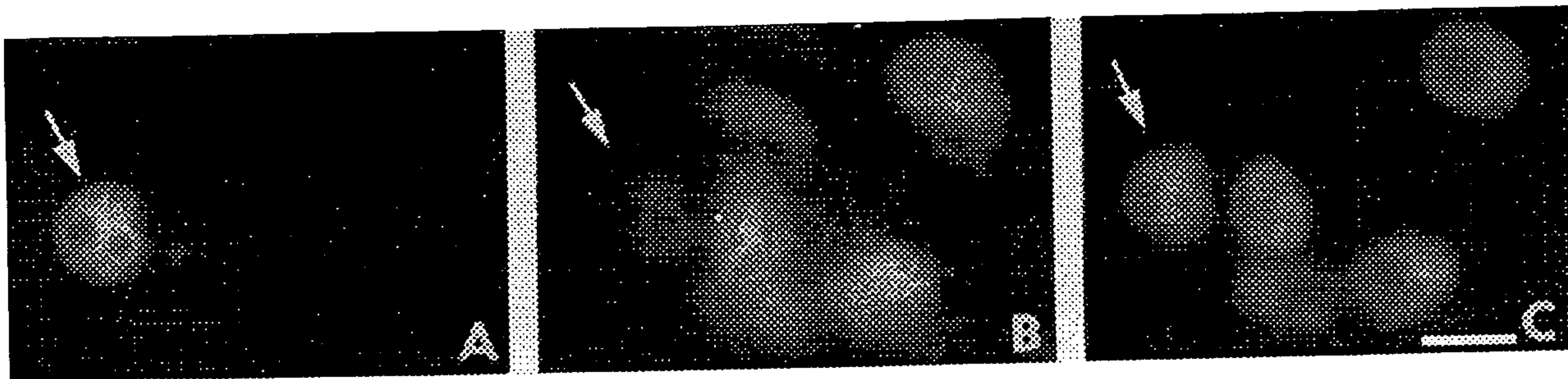
Figure 8: Immunofluorescence in situ detection of DNA double strands breaks in cells of V. faba . Cells were stained with: FITC for DNA breaks labeling, chromatin binding dye DAPI. A-B: DNA breaks labeling, B: chromatin binding dye DAPI, A-B: DNA breaks labeling in nuclei after 12h of 25 treatment, chromatin already with apoptotic fragmentation (arrow). C apoptotic nuclei with condensed globular chromatin domains.
