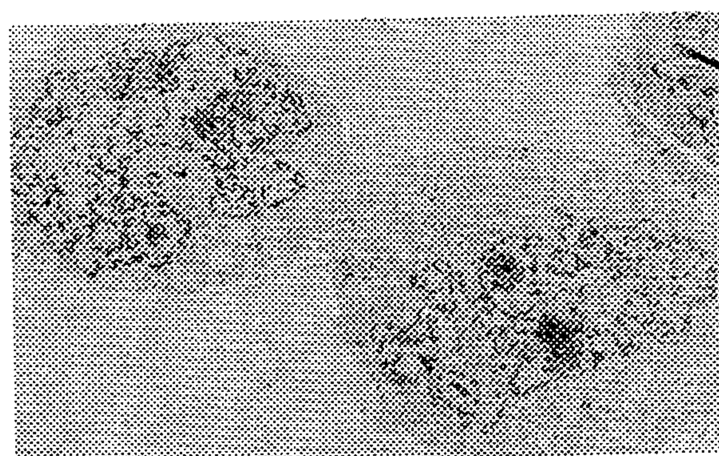
isopentenyladenine
