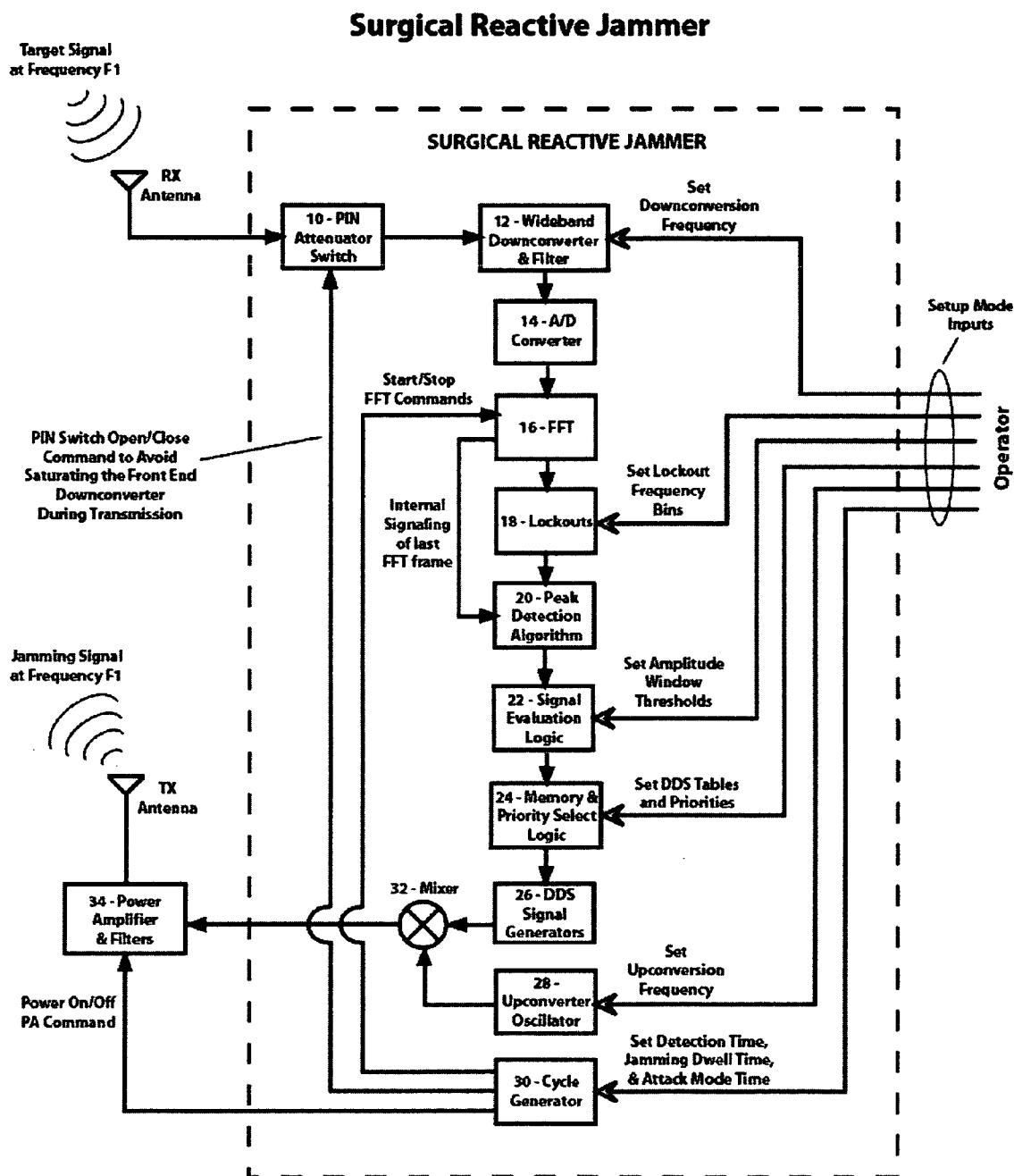
FIGURE 1 – PRIOR ART
