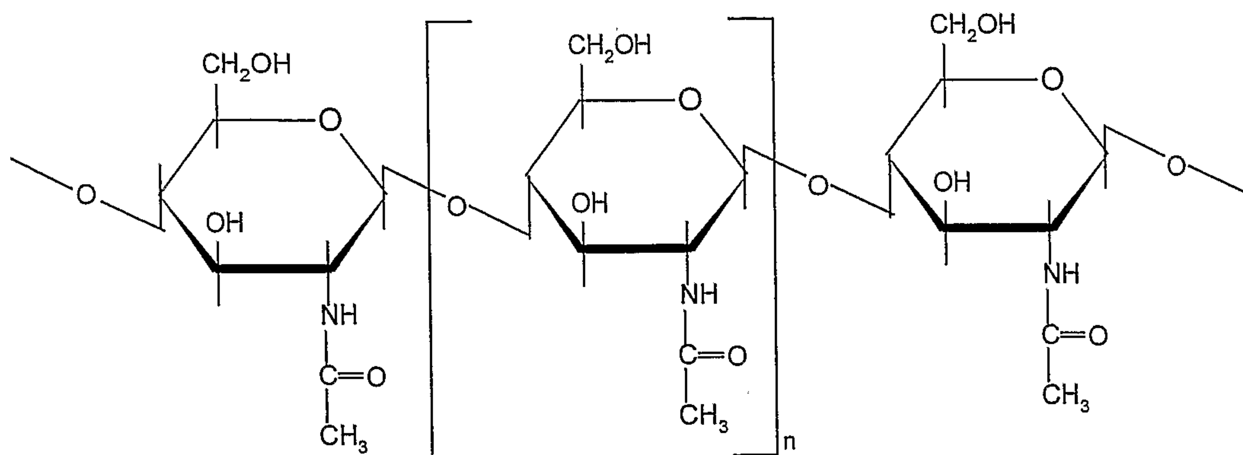
Scheme 1. Structure of fully acetylated chitin (poly N -acetyl-D-glucosamine).
