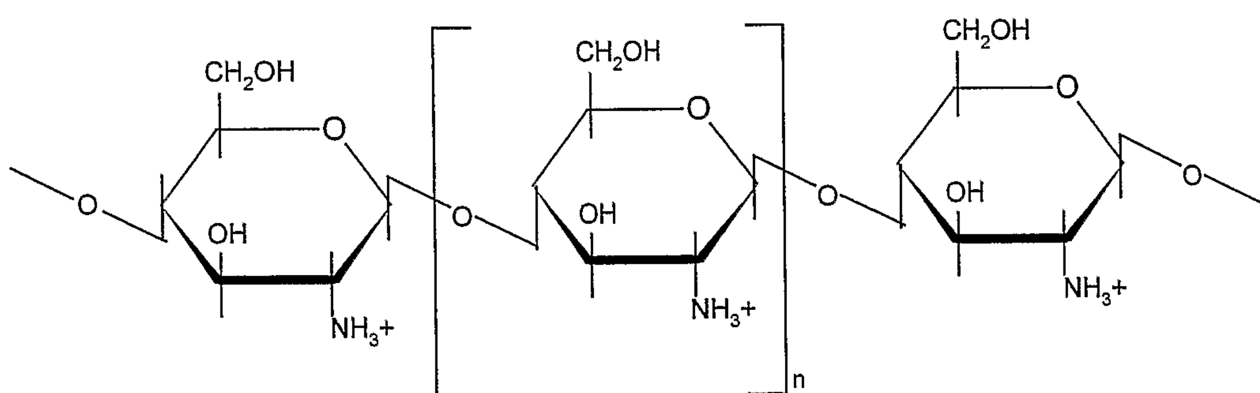
Scheme 2. Structure of fully deacetylated chitosan (poly D-glucosamine, protonated form at low pH).
