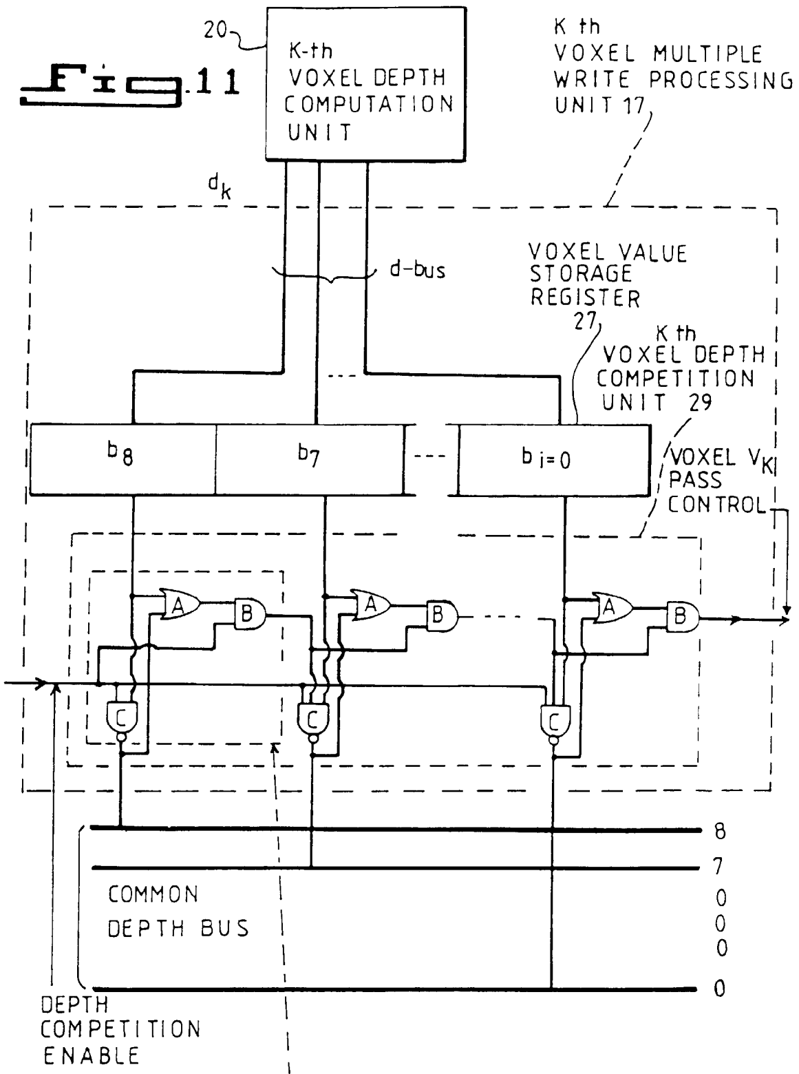
VOXEL DEPTH BIT VALUE ( b_i ) COMPARISON LOGIC FOR FIRST STAGE OF DEPTH BIT COMPETITION
