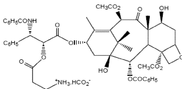
2'-B-Alanyl-Taxol Formate
