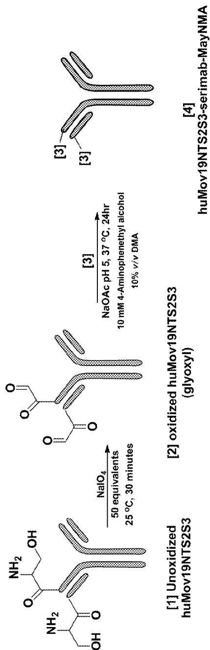
Scheme 7
