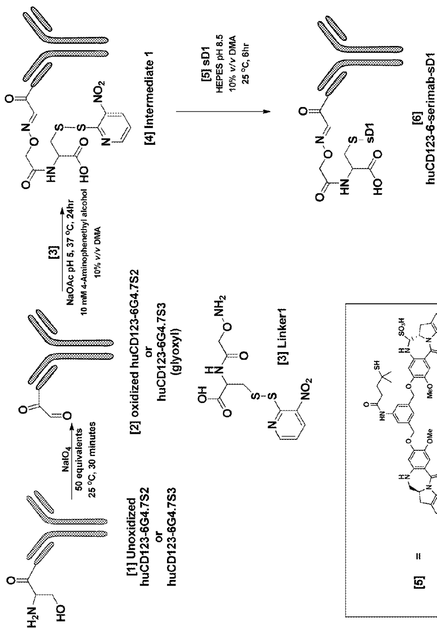
Scheme 5
