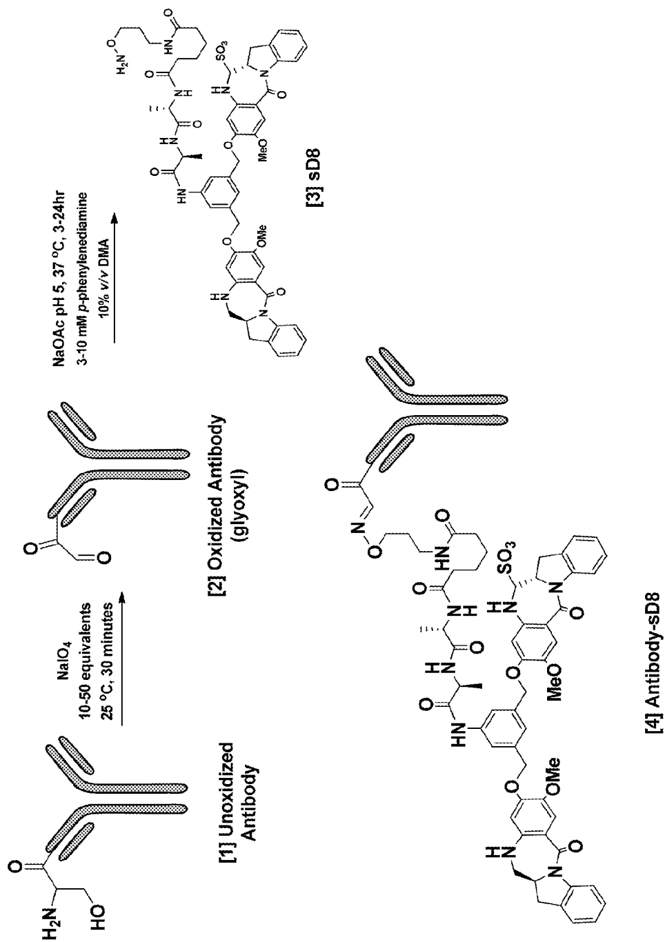
Scheme 4
