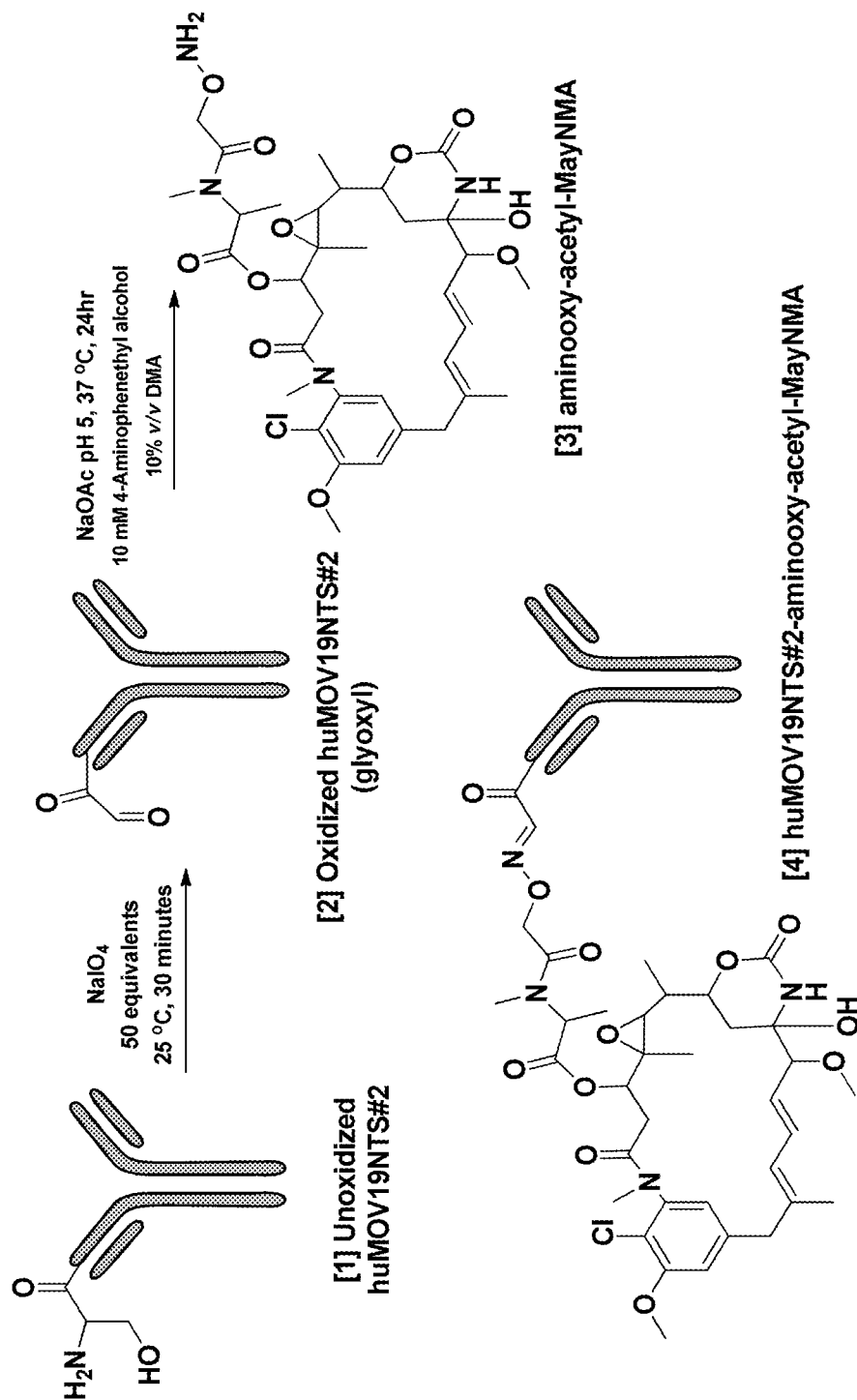
Scheme 2
