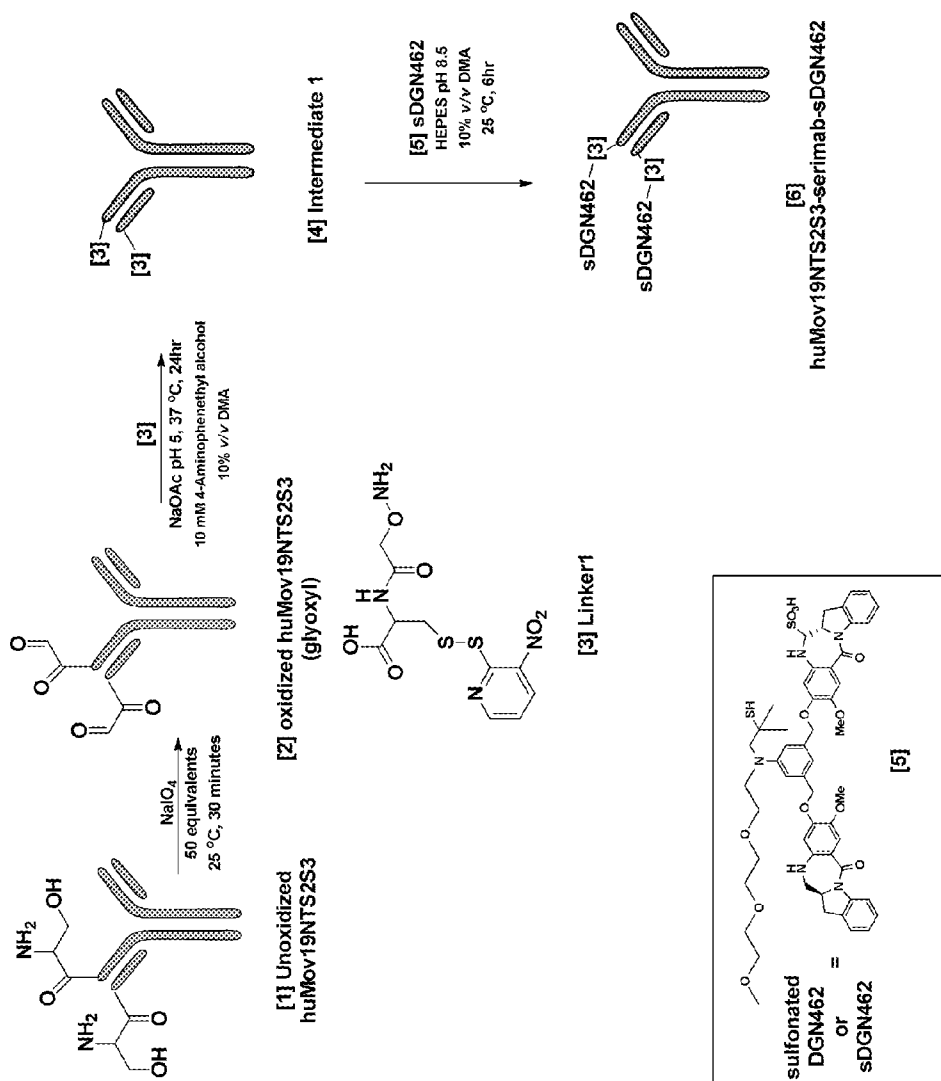
Scheme 6
