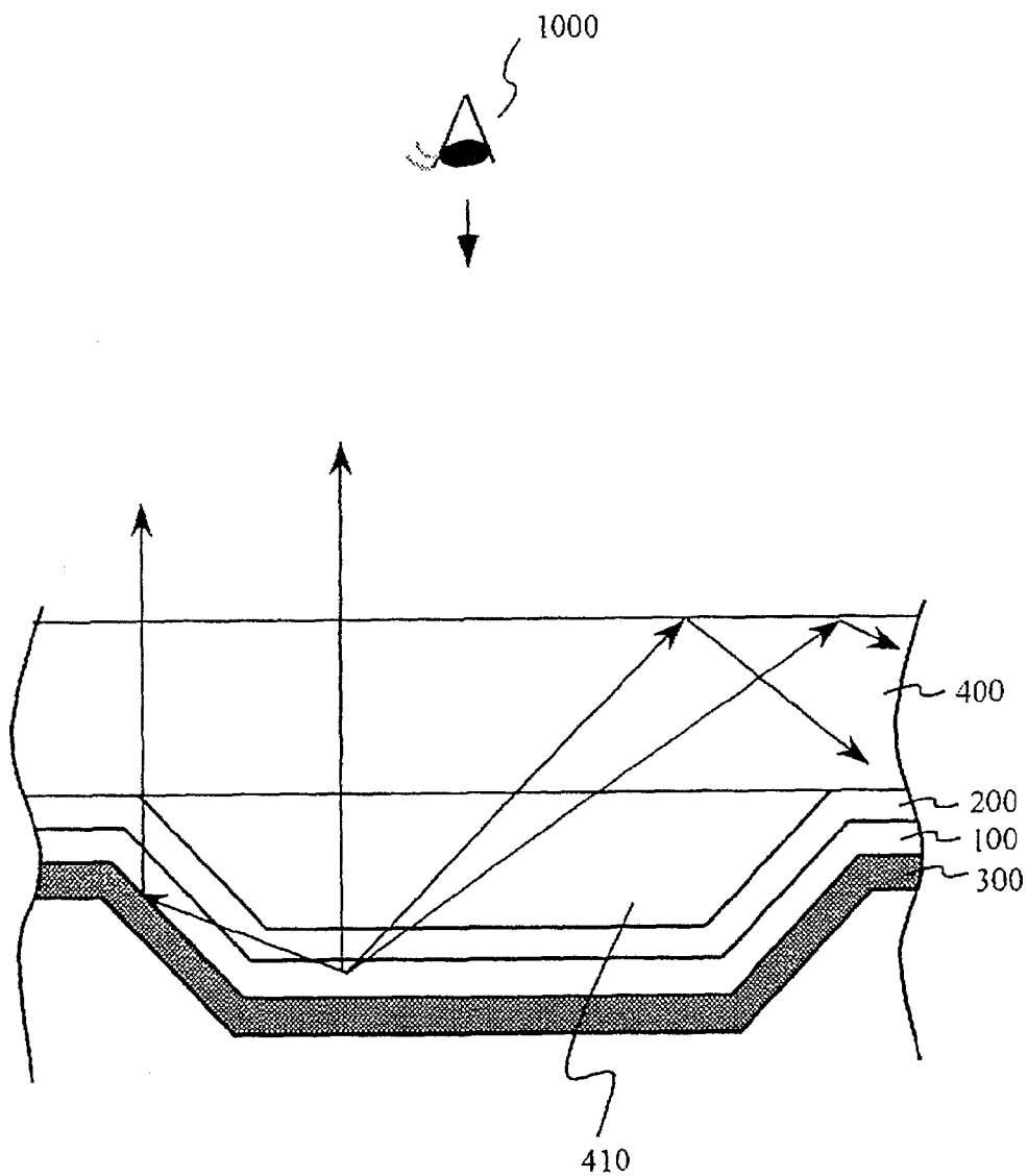
FIG. 34 PRIOR ART
