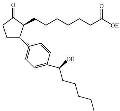
(1S, 2R)-2-[4-(1-(S)-hydroxyhexyl)phenyl]- 5-oxo-cyclopentaneheptanoic acid [SRS]
