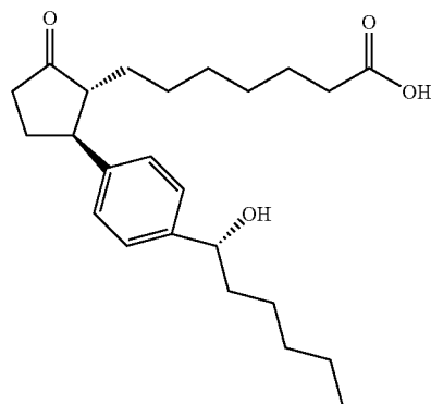
(1R, 2S)-2-[4-(1-(R)-hydroxyhexyl)phenyl]- 5-oxo-cyclopentaneheptanoic acid [RSS]
