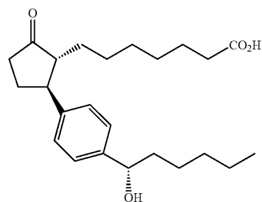
Peak 1, mixture 1 (FIG. 7a-C)
