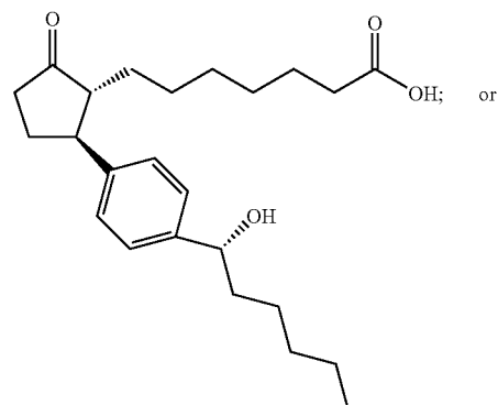
(1R, 2S)-2-[4-(1-(R)-hydroxyhexyl)phenyl]-5-oxo-cyclopentaneheptanoic acid [RSR]
