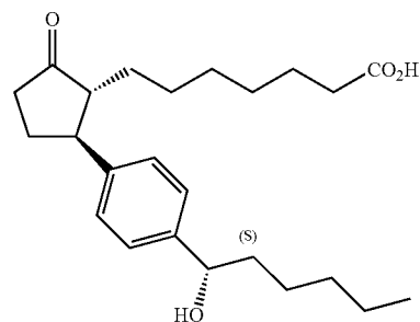
Peak 1, mixture 1 acid (C) (1R,2S)-2-[4-(1-(S)-hydroxyhexyl)phenyl]- 5-oxo-cyclopentaneheptanoic acid
