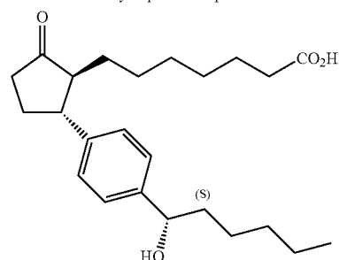
Peak 2, mixture 1 acid (A) (1S,2R)-2-[4-(1-(S)-hydroxyhexyl)phenyl]- 5-oxo-cyclopentaneheptanoic acid
