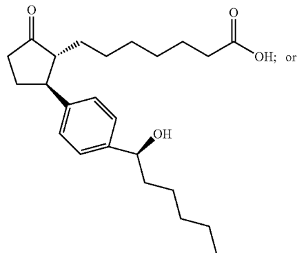
(1R, 2S)-2-[4-(1-(S)-hydroxyhexyl)phenyl]- 5-oxo-cyclopentaneheptanoic acid [RSS]
