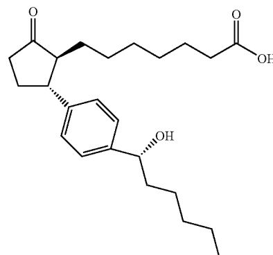
(1S, 2R)-2-[4-(1-(R)-hydroxyhexyl)phenyl]-5-oxo-cyclopentaneheptanoic acid [SRR]
