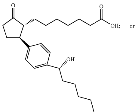
(1R, 2S)-2-[4-(1-(R)-hydroxyhexyl)phenyl]- 5-oxo-cyclopentaneheptanoic acid [RSS]
