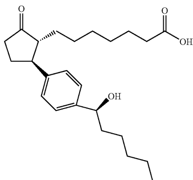
(1R,2S)-2-[4-(1-(S)-hydroxyhexyl)phenyl]-5-oxo-cyclopentaneheptanoic acid [RSS]
