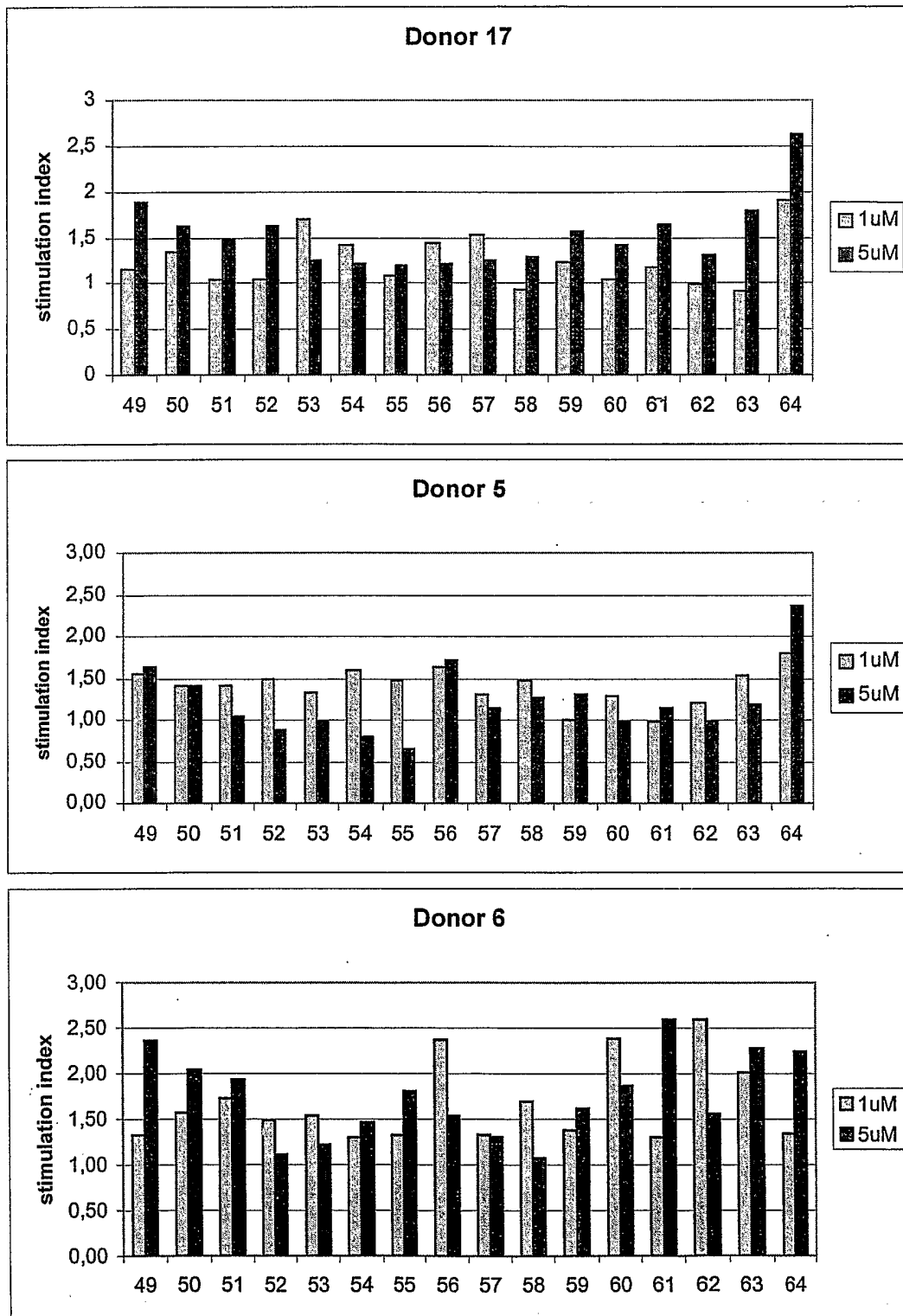
PBMC donor response charts to bryodin 1 peptides #49 - 64 Peptide #64 is encompassed within epitope region R5
