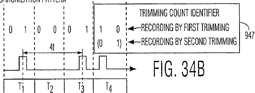
FIXED SYNCHRONIZATION PATTERN
