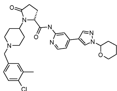
F2 UPLC ( R_t ) = 1.69 min method M
