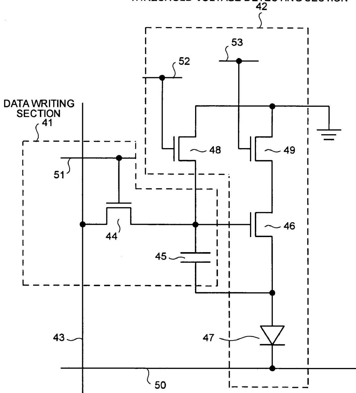
THRESHOLD VOLTAGE DETECTING SECTION
