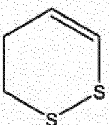
3,4-dihydro-1,2-dithiine
