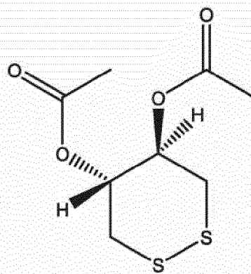
(4R,5R)-1,2-dithian-4,5-diyl diacetate
