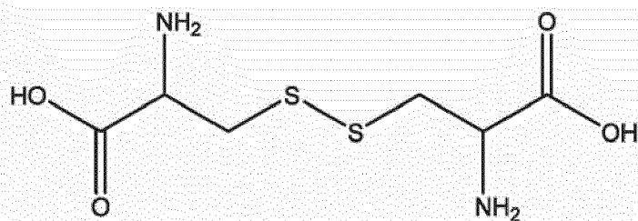
cystine
