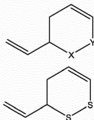
3-vinyl-[4H]-1,2-dithiine
