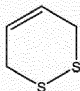
3,6-dihydro-1,2-dithiine
