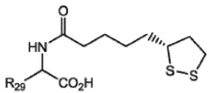
Formula IVB
