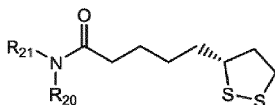
Formula III(R).
