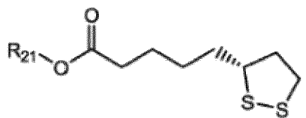
Formula VI(R).
