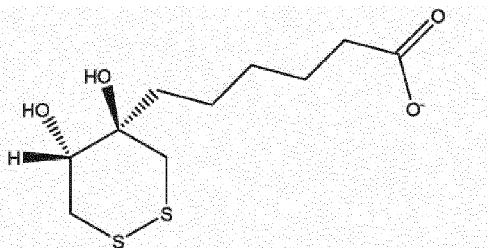
6-((4R,5R)-4,5-dihydroxy-1,2-dithian-4-yl) hexanoate
