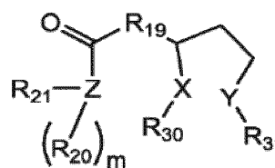
Formula I-NC
