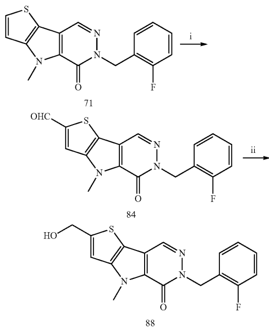
Scheme 7
