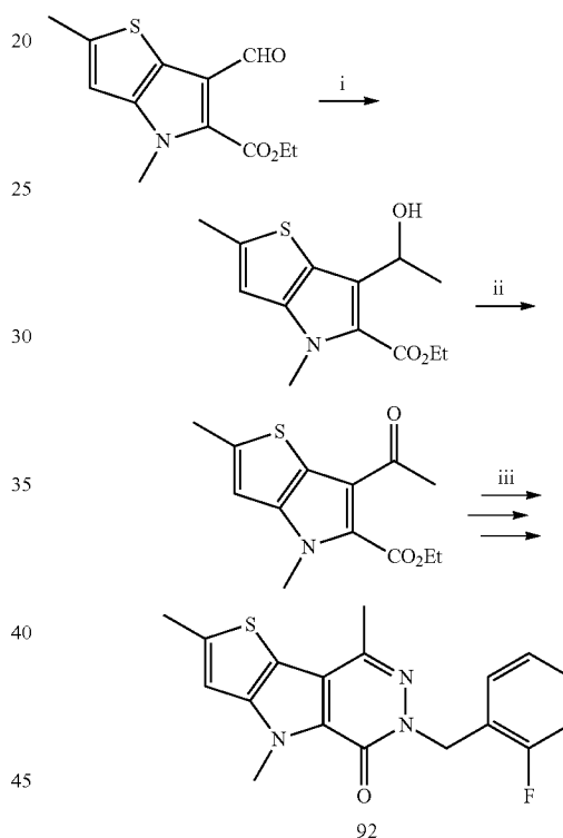
Scheme 8
