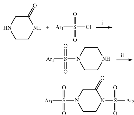
Scheme 3
