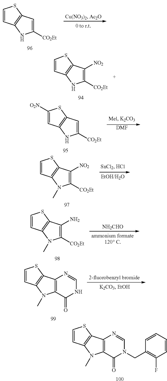
Ethyl-6-amino-4-methyl-4H-thieno[3,2-b]pyrrole-5-carboxylate (98)
