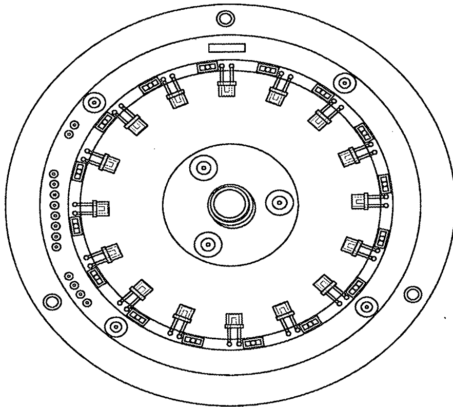
Figure. 6A (Prior Art)
