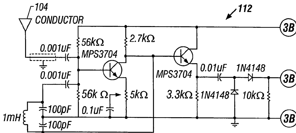
Y-Axis Proximity Detector
