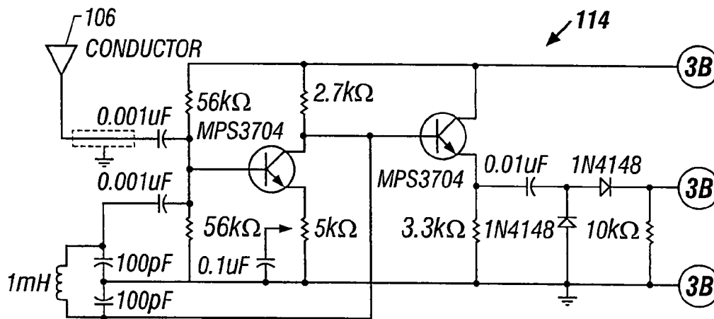
Z-Axis Proximity Detector
