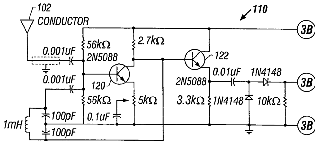
X-Axis Proximity Detector
