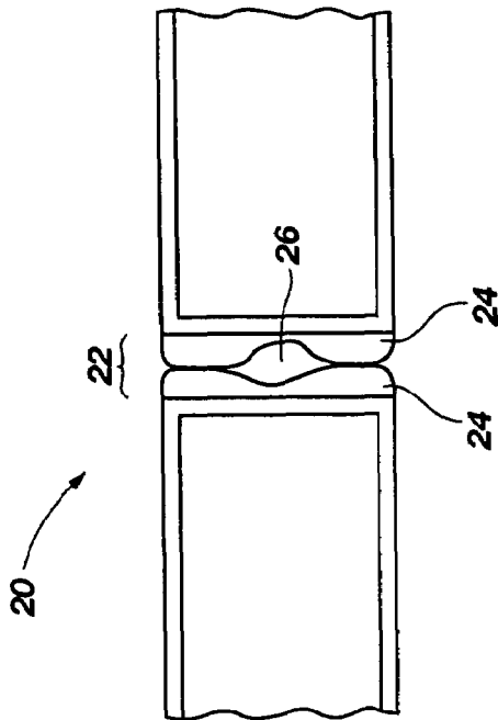
FIG. 2 (PRIOR ART)
