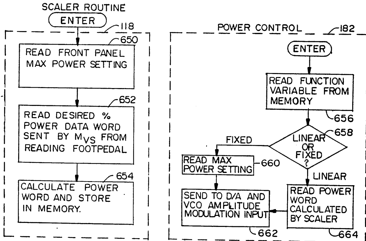
FIG. 29 POWER CONTROL
