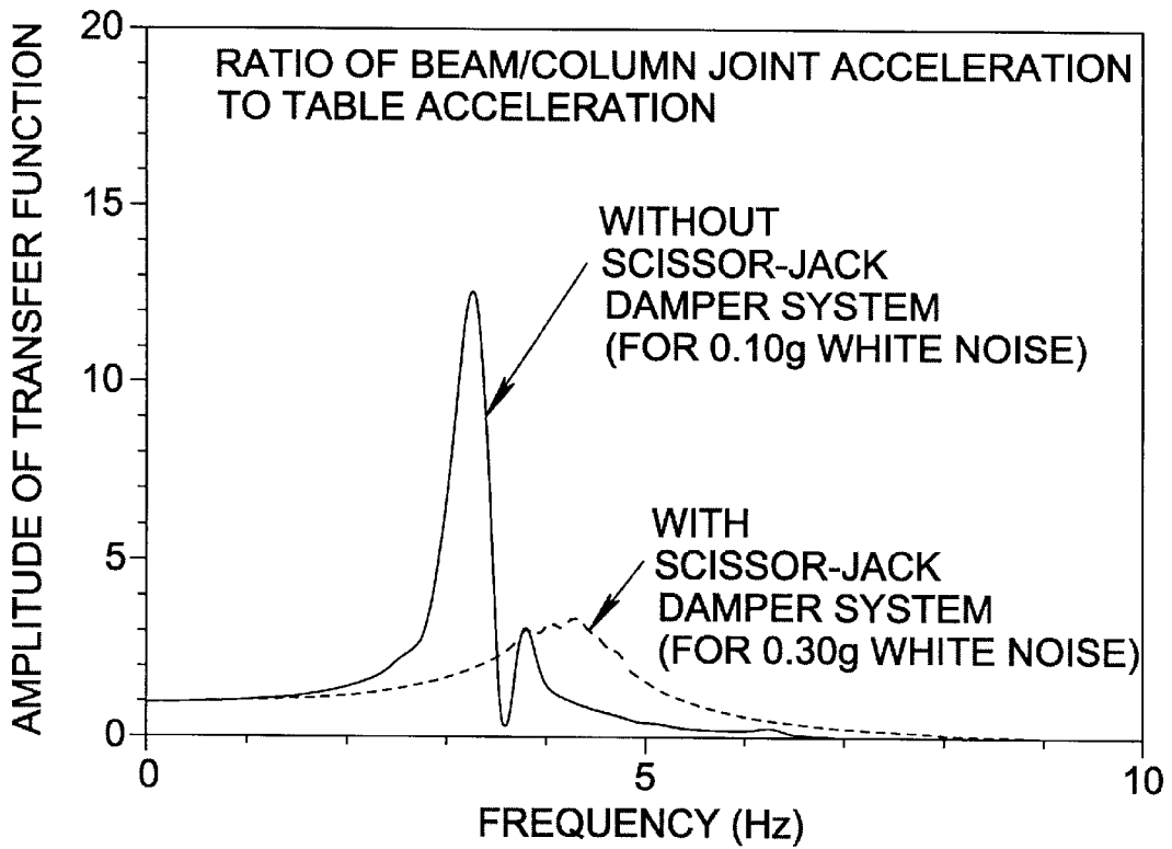
AMPLITUDE OF TRANSFER FUNCTION OF TESTED STRUCTURE WITH AND WITHOUT SCISSOR-JACK DAMPER SYSTEM
