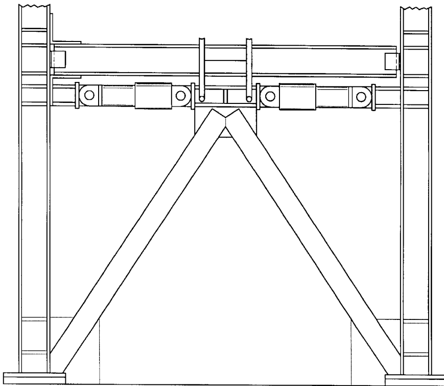
FIG. 2 - PRIOR ART
