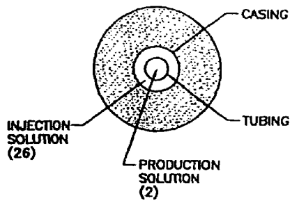
FIGURE 3A CROSS SECTION DETAIL A-A'
