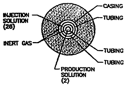
FIGURE 3C CROSS SECTION DETAIL A-A'
