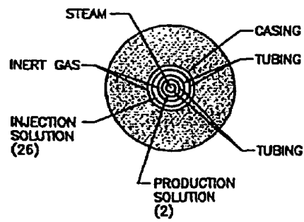
FIGURE 3D CROSS SECTION DETAIL A-A'
