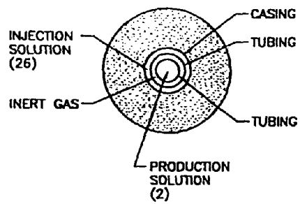
FIGURE 3B CROSS SECTION DETAIL A-A'
