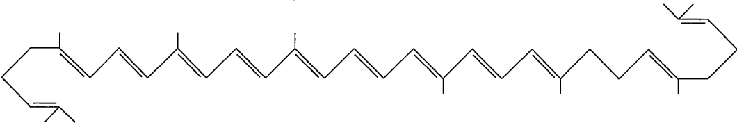
NEUROSPORENE
