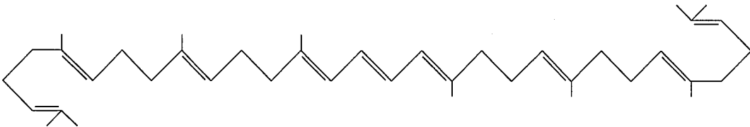
PHYTOENE
