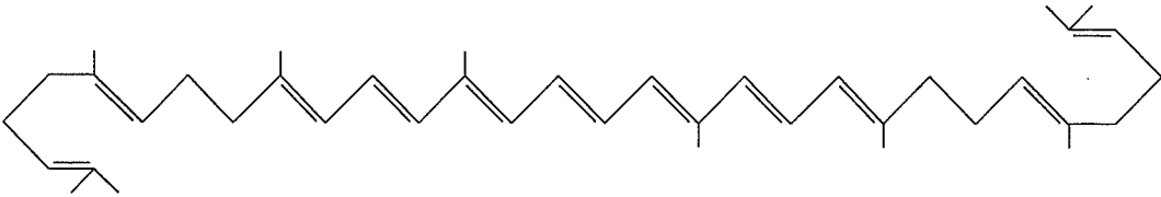
\zeta -CAROTENE
