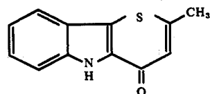
2-Methylthiopyrano[3,2-b]indol-4(5H)-one.
