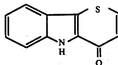
Thiopyrano[3,2-b]indol-4(5H)-one.
