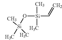
Pentamethylvinylsiloxane (CAS: 1438-79-5)
