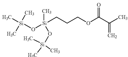
3-Methacryloxypropylheptamethyltrisiloxane (CAS: 19309-90-1)
