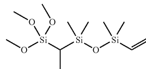
1-Vinyl-3-(1-trimethoxysilylethyl)- 1,1,3,3-tetramethyldisiloxane
