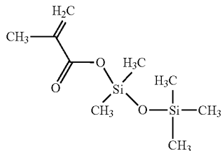
Pentamethyldisiloxanyl methacrylate (CAS: 4880-04-0)
