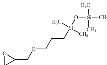
3-Glycidyloxypropylpentamethyldisiloxane (CAS: 18044-44-5)
