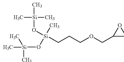
3-Glycidyloxypropyl heptamethyltrisiloxane (CAS: 7422-52-8)
