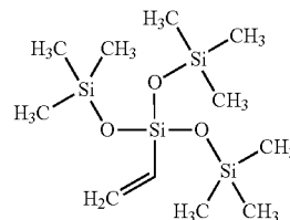
Vinyltris(trimethylsiloxy)silane (CAS: 5356-84-3)
