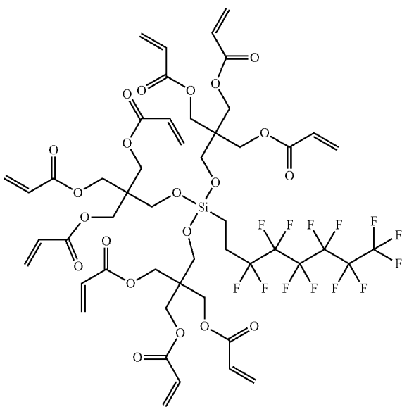
[2-[[bis[3-prop-2-enoyloxy-2,2-bis(prop-2-enoyloxymethyl)propoxy]-(3,3,4,4,5,5,6,6,7,7,8,8,8-tridecafluorooctyl)silyl]oxymethyl]-3-prop-2-enoyloxy-2-(prop-2-enoyloxymethyl)propyl] prop-2-enoate (CAS: 94237-13-5)
