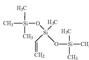
3-Vinylheptamethyltrisiloxane (CAS: 5356-85-4)
