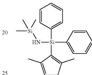
[(2,5-dimethylcyclopenta-1,4-dien-1-yl)-phenyl-(trimethylsilylamino)silyl]benzene
