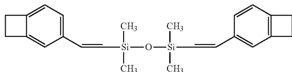
1,3-bis(2-bicyclo[4.2.0]octa-1,3,5-trien-3-yl ethenyl)-1,1,3,3 tetramethyldisiloxane
