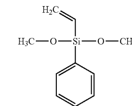
Phenylvinyl dimethoxysilane (CAS: 20151-57-9)
