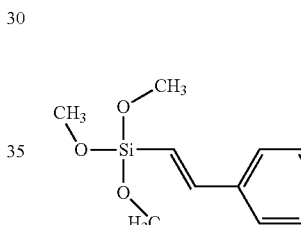
(E)-1-Phenyl-2-trimethoxysilylethene (CAS: 70531-02-1)
