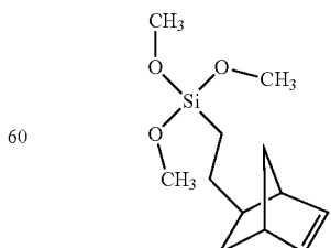
Norbornenylethyltrimethoxysilane (CAS: 68245-19-2)
