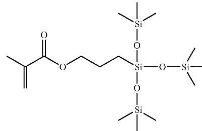
Methacryloxypropyltris(trimethylsiloxy)silane (CAS: 17096-07-0)
