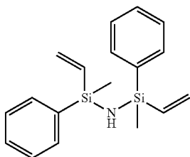
1,4-divinyl-1,3-diphenyl-1,3-dimethyldisilazane (CAS: 23038-10-0)
