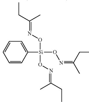
Phenyltris(methylethylketoxime)silane (CAS: 34036-80-1)
