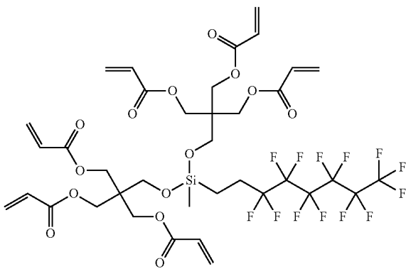
[2-[[methyl-[3-prop-2-enoyloxy-2,2-bis(prop-2-enoyloxymethyl)propoxy]- (3,3,4,4,5,5,6,6,7,7,8,8,8-tridecafluorooctyl)silyl] oxymethyl]-3-prop-2-enoyloxy-2-(prop-2- enoyloxymethyl)propyl] prop-2-enoate (CAS: 94237-12-4)
