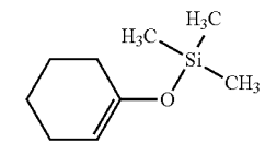
Trimethylsilyloxy-1-cyclohexene (CAS: 6651-36-1)
