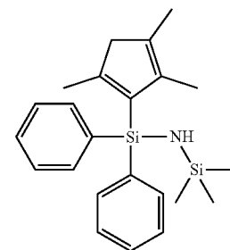
[phenyl-(2,4,5-trimethylcyclopenta-1,4-dien-1-yl)-(trimethylsilylamino)silyl]benzene
