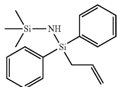
[phenyl-prop-2-enyl-(trimethylsilylamino)silyl]benzene
