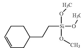
2-(3-Cyclohexenyl)ethyltrimethoxysilane (CAS: 67592-36-3)
