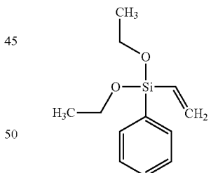
Phenylvinyl diethoxysilane (CAS: 4652-09-9)
