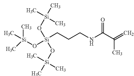
Tris(trimethylsiloxy) silylpropylmethacrylamide (CAS: 115257-95-9)
