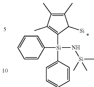
[2-[diphenyl-trimethylsilylamino)silyl]-3,4,5-trimethylcyclopenta-2,4-dien-1-yl]silicon
