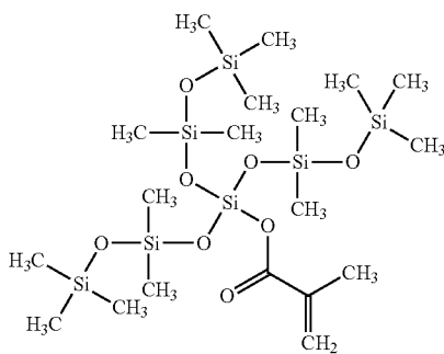
3-Methacryloxypropyltris (pentamethyldisiloxy)silane (CAS: 60734-89-5)
