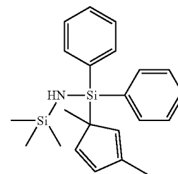
[(1,3-dimethylcyclopenta-2,4-dien-1-yl)-phenyl-(trimethylsilylamino)silyl]benzene
