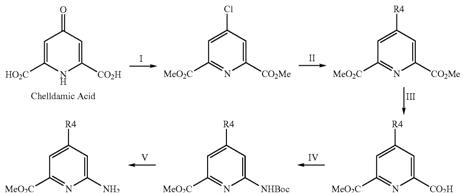
Reaction scheme 9:
