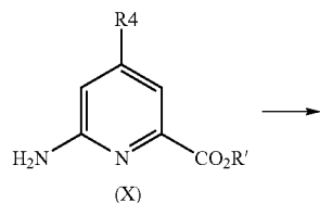
Reaction scheme 3:
