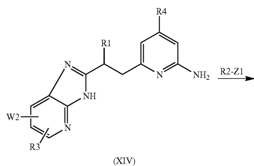
Reaction scheme 7:
