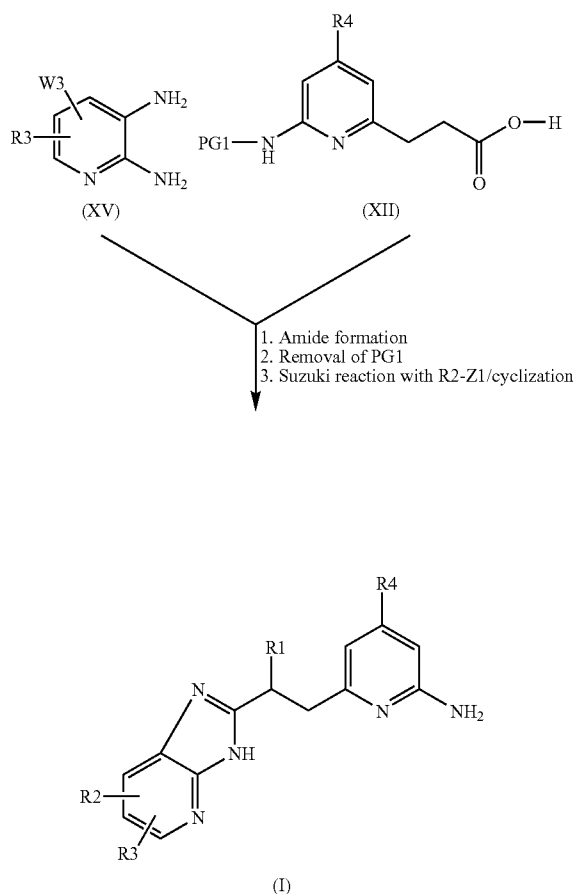
Reaction scheme 8:
