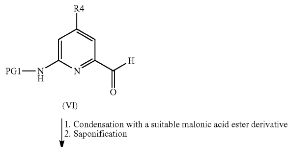
Reaction scheme 6:
