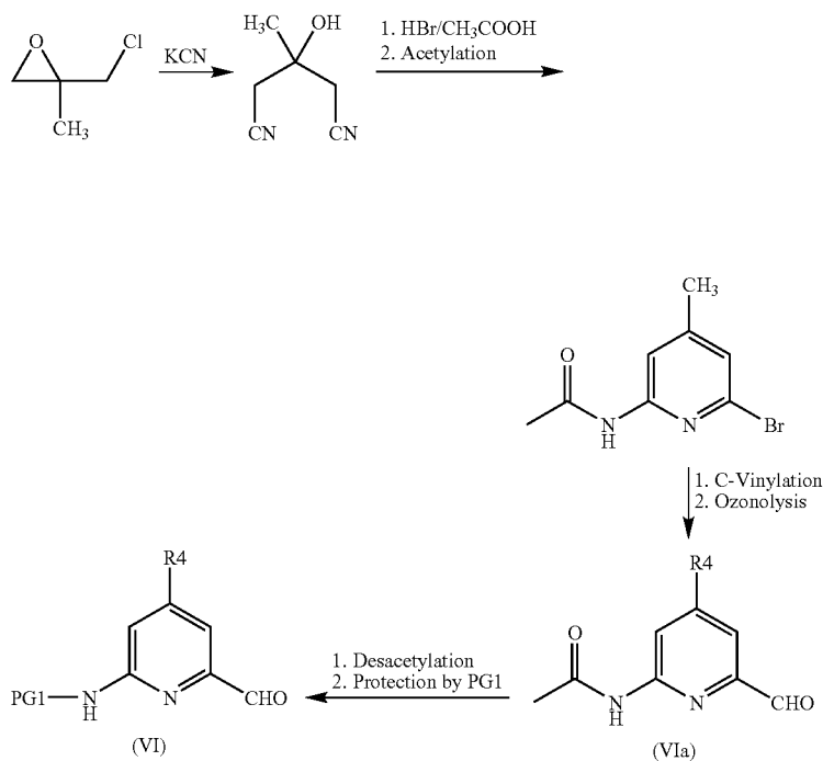
Reaction scheme 5:
