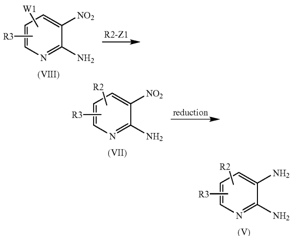
Reaction scheme 2:
