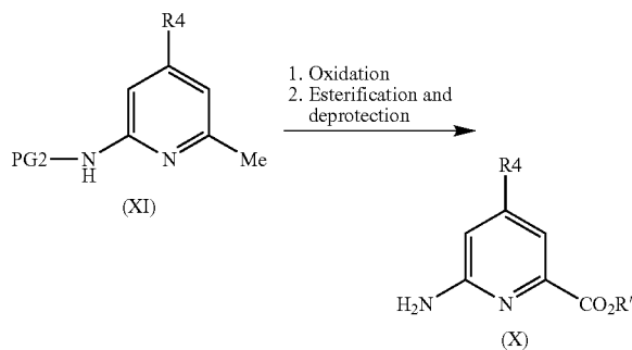
Reaction scheme 4:
