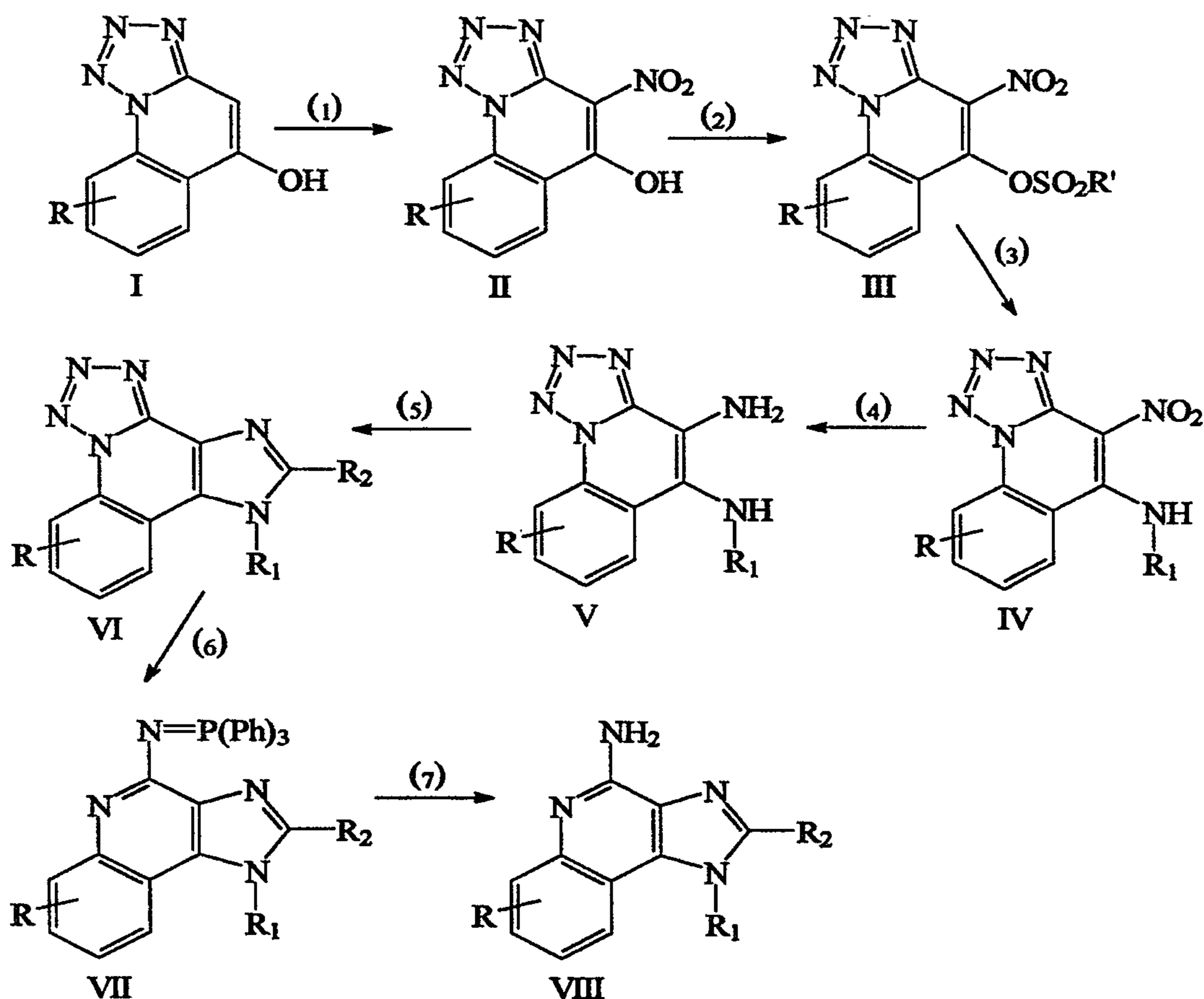
Reaction Scheme I
