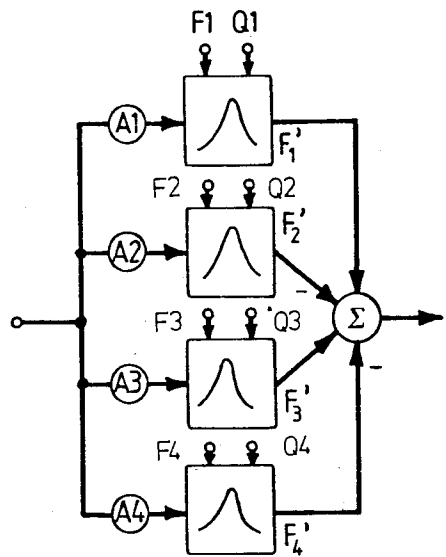
FIG. 1B Parallel Model (Prior Art)
