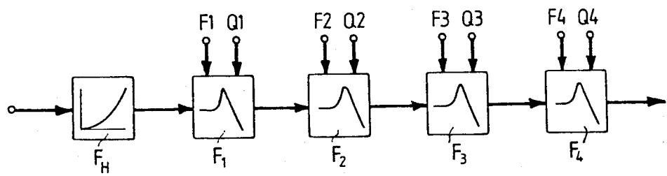
FIG. 1A Cascaded Model (Prior Art)
