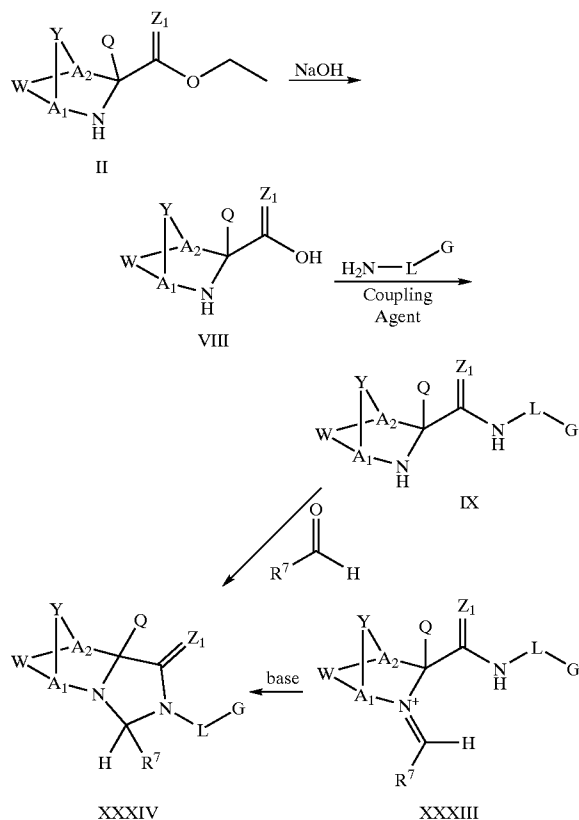
Scheme XII
