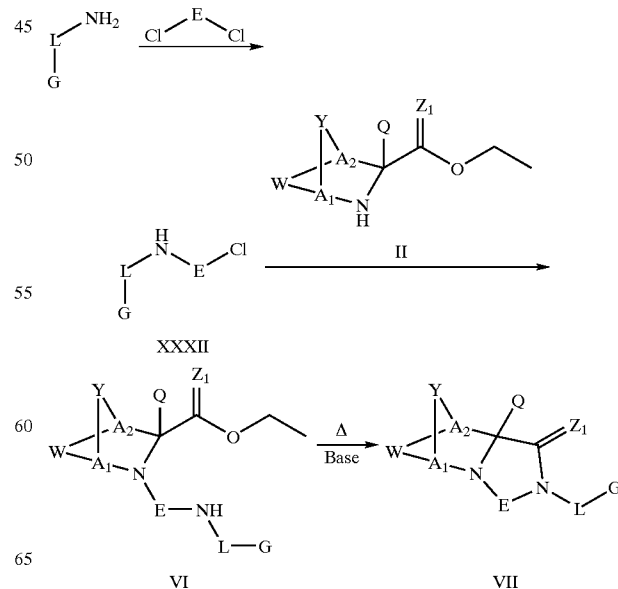
Scheme XI
