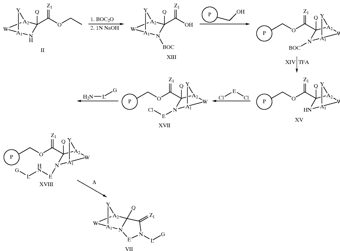
Scheme VII
