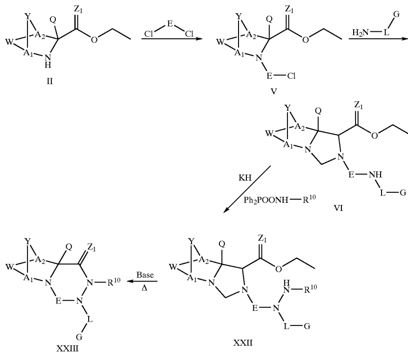
Scheme VIII
