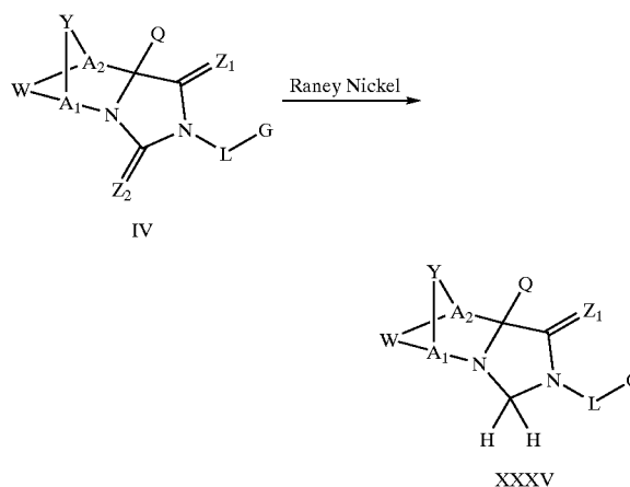
Scheme XIII
