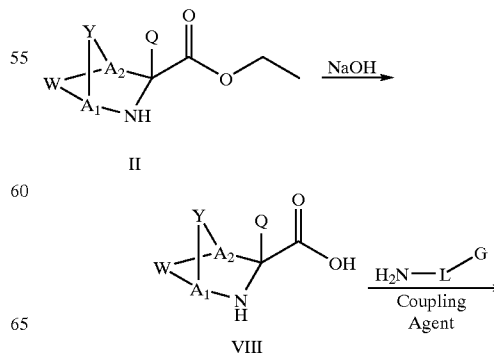
Scheme XIV
