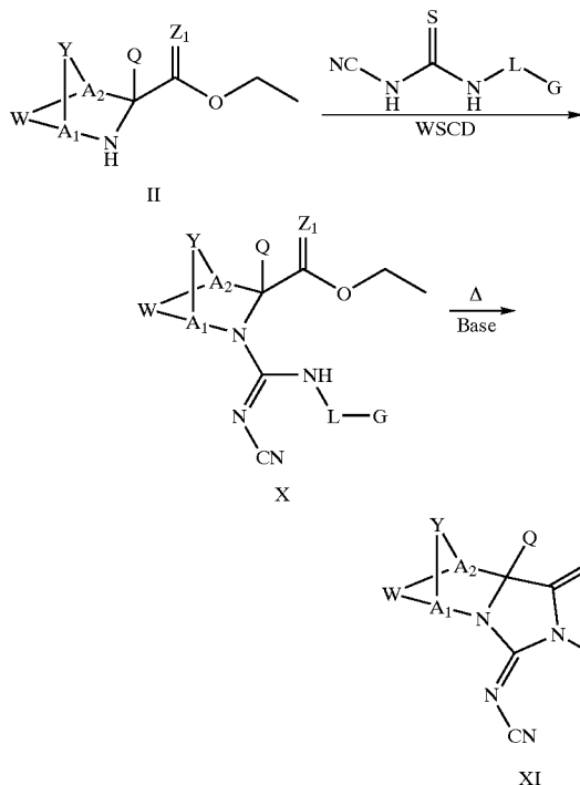
Scheme IV
