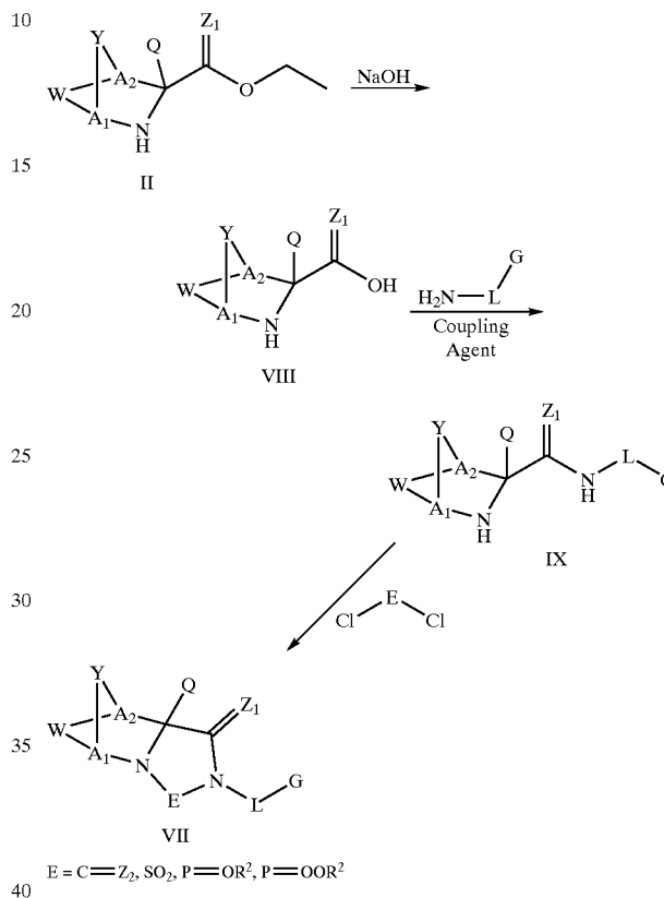
Scheme III
