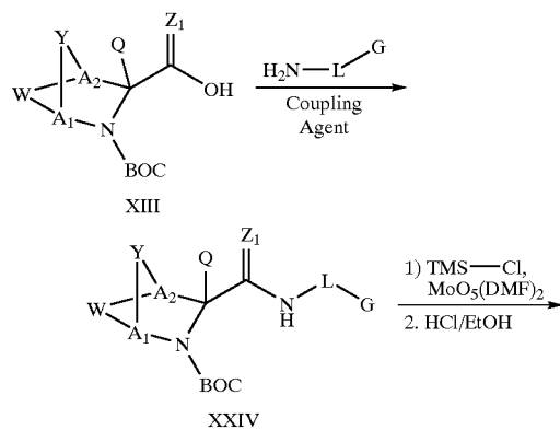
Scheme X
