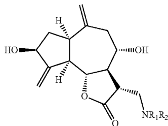
Aminodesacylcynaropicrins
