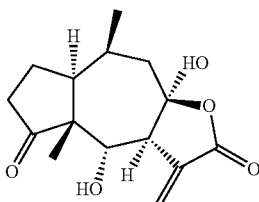
11,13-Dihydrohelenalin
