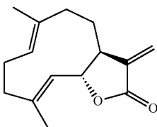
Costunolide
