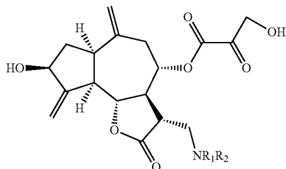
Aminocynaropicrins
