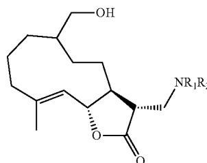
Aminosoulangianolides
