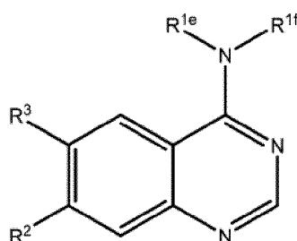
Formel II
