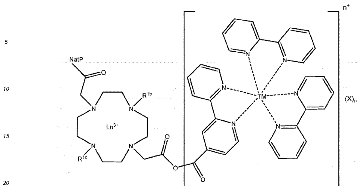
Formel H
