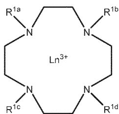
Formula D
