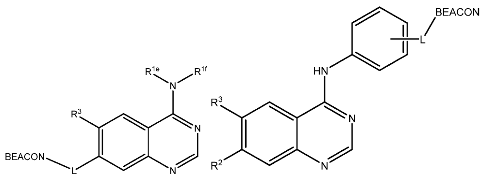
Formula III
