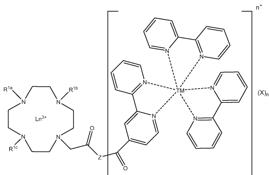
Formula A
