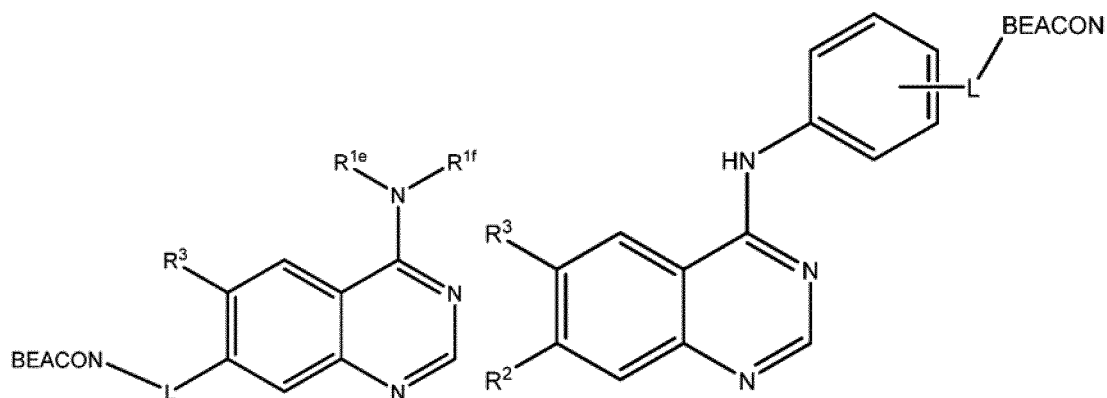
Formel III
