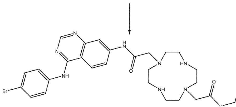
ethyl 2-(7-(2-((4-(4-bromophenyl)amino)quinazolin-7-yl)amino)-2-oxoethyl)-1,4,7,10-tetraazacyclododecan-1-yl)acetate
