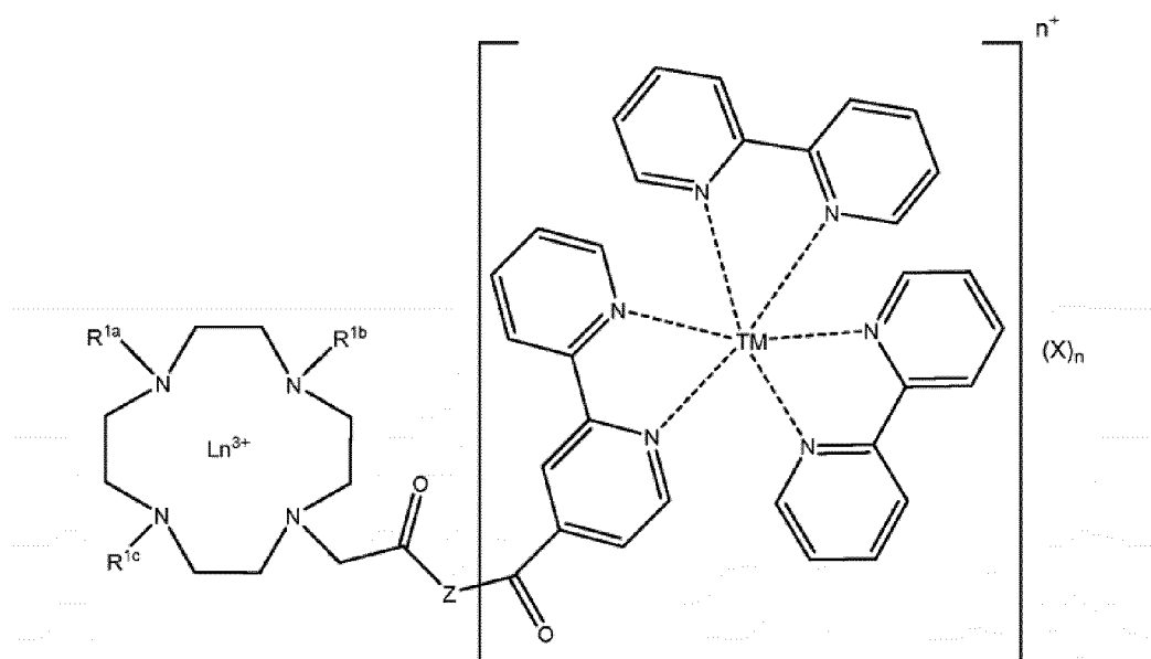
Formel A
