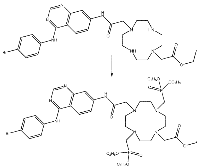
ethyl 2-(7-(2-((4-bromophenyl)amino)quinazolin-7-yl)amino)-2-oxoethyl)-4,10-bis((diethoxyphosphoryl)methyl)-1,4,7,10-tetraazacyclododecan-1-yl)acetate
