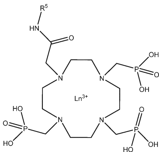
Formula Fa
