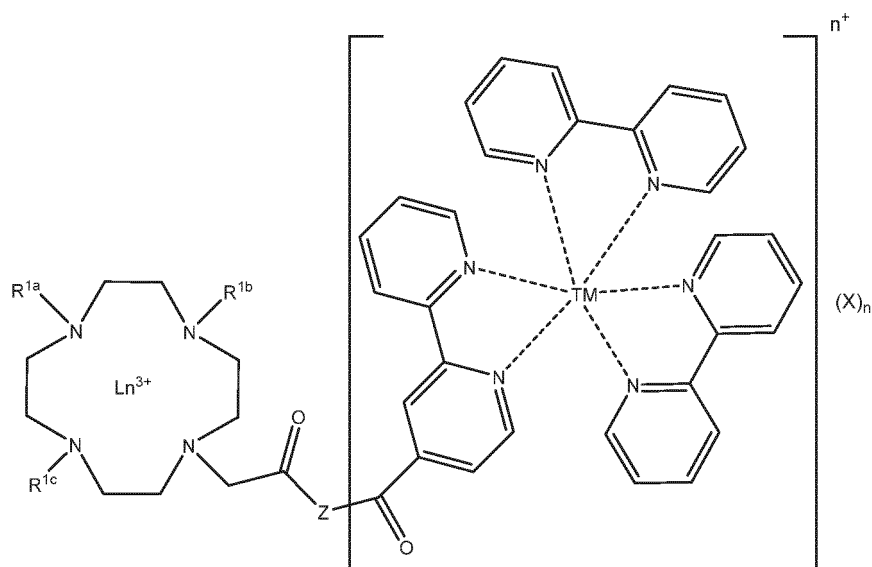
Formula A
