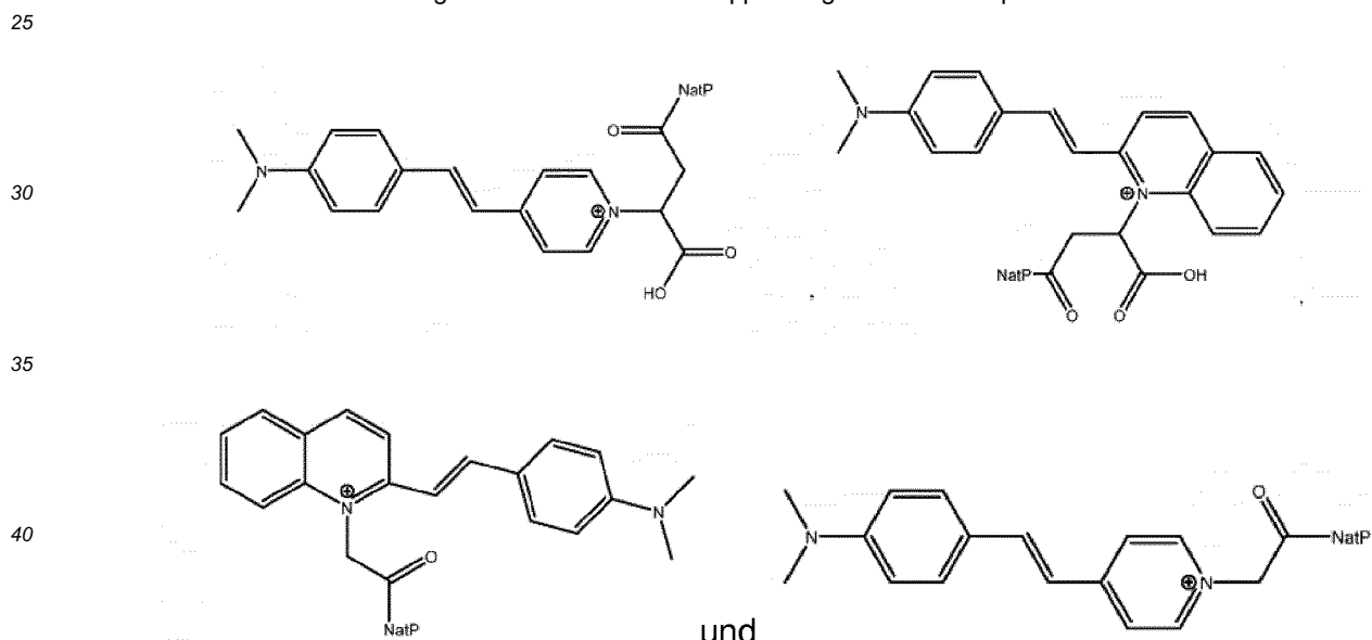
Formel H
