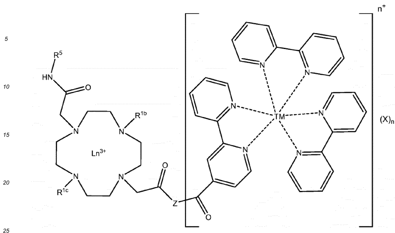
Formel B
