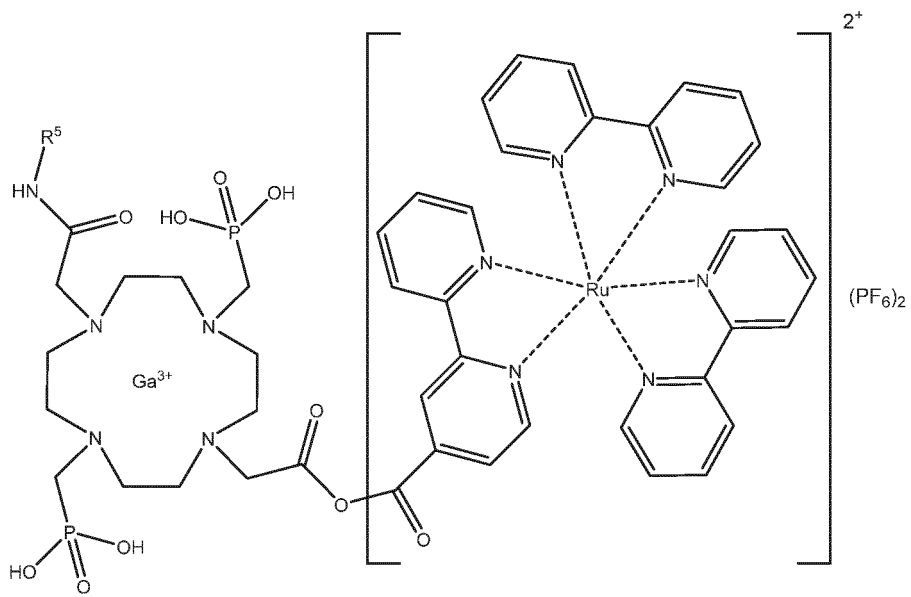
Formula C
