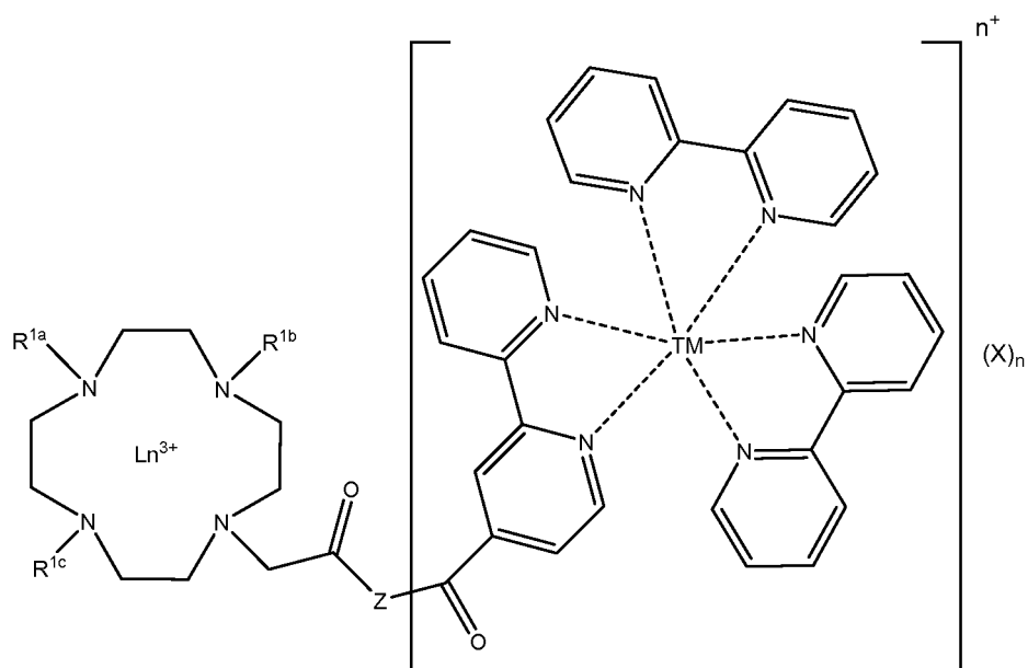
Formula A
