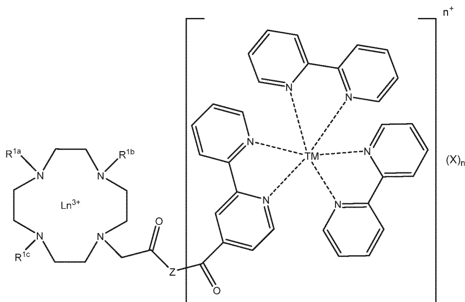
Formula A
