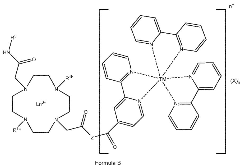
Formula B
