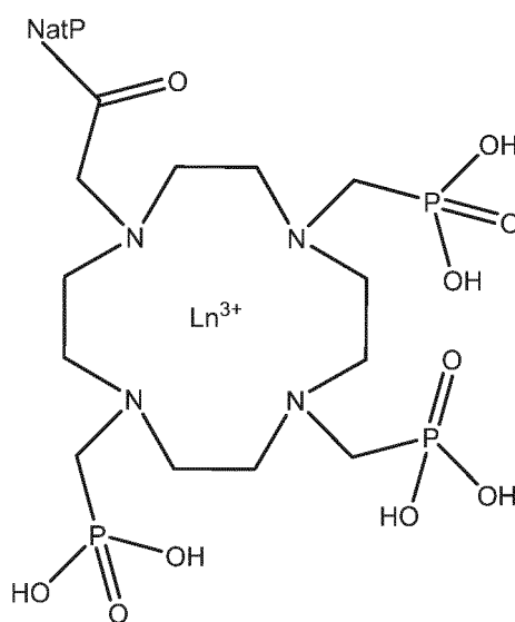
Formula G
