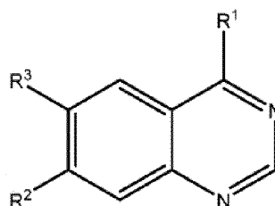
Formel I
