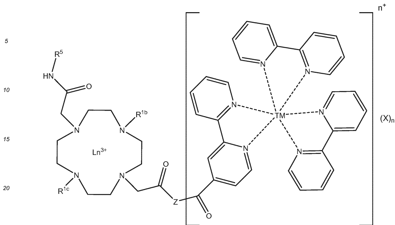
Formula B
