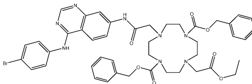
dibenzyl 4-(2-((4-((4-bromophenyl)amino)quinazolin-7-yl)amino)-2-oxoethyl)-10-(2-ethoxy-2-oxoethyl)-1,4,7,10-tetraazacyclododecane-1,7-dicarboxylate
