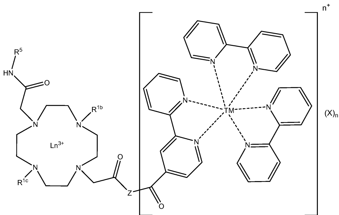
Formula B
