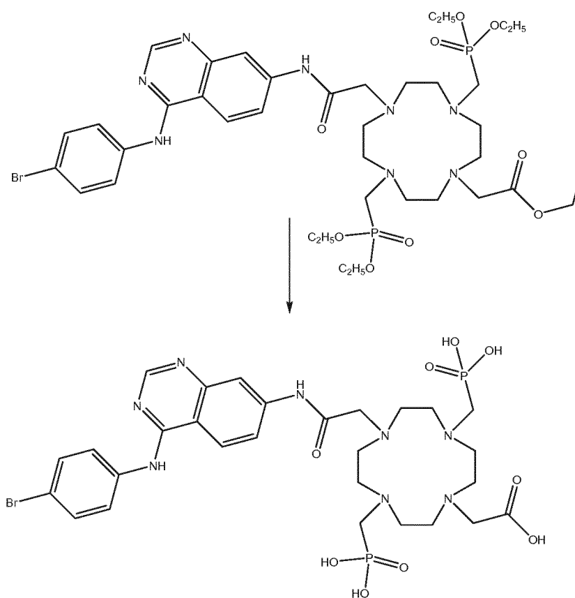
2-(7-(2-((4-(4-bromophenyl)amino)quinazolin-7-yl)amino)-2-oxoethyl)-4,10-bis(phosphonomethyl)-1,4,7,10-tetraazacyclododecan-1-yl)acetic acid
