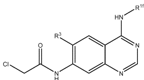
Formula IIa
