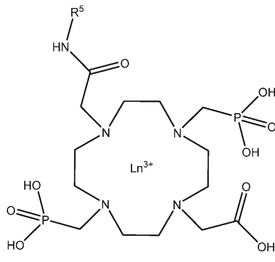
Formula Fb
