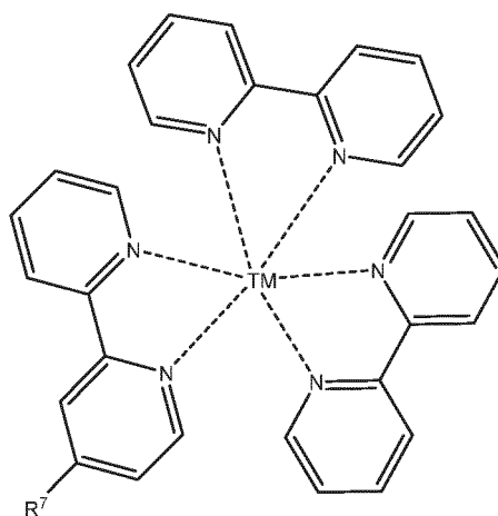
Formula E
