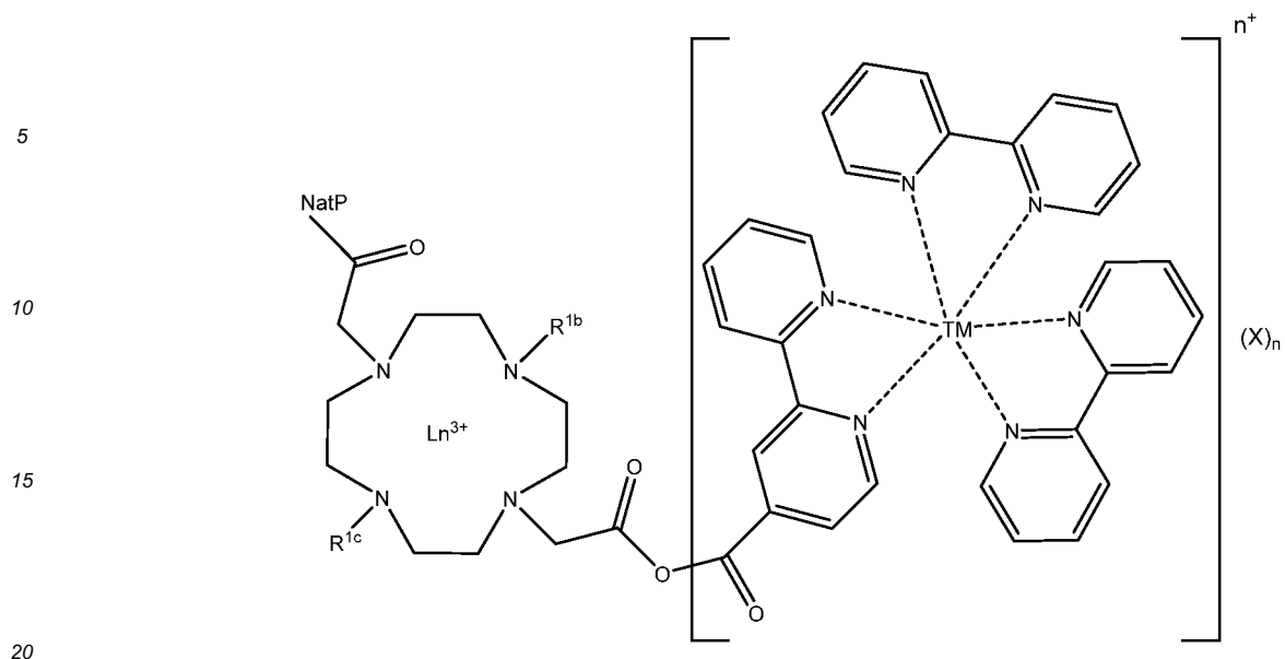
Formula H
