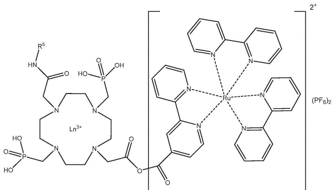
Formula C
