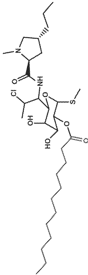
Clindamycin Lauric Acid Conjugate
