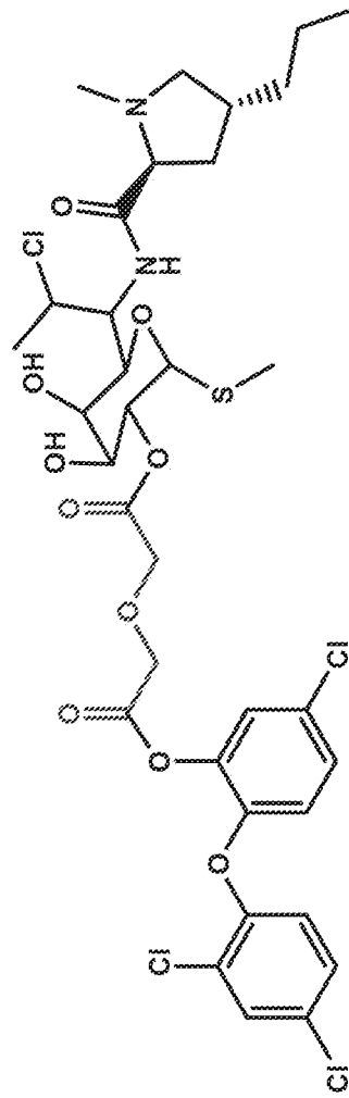
Clindamycin Triclosan with Oxylacetic Acid
