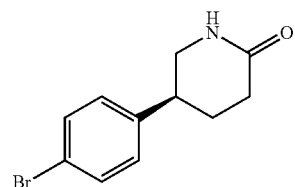
(S)-5-(4-bromophenyl)piperidin-2-one
