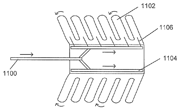
pushing rod collapses bristles
