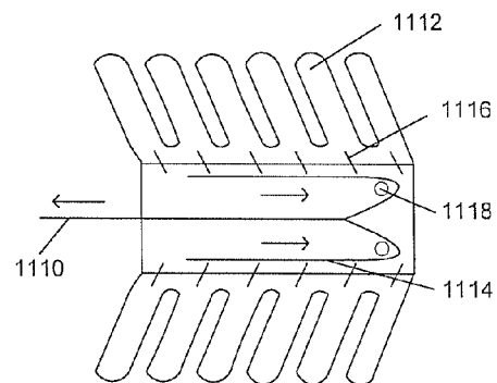
Pulling string collapses bristles
