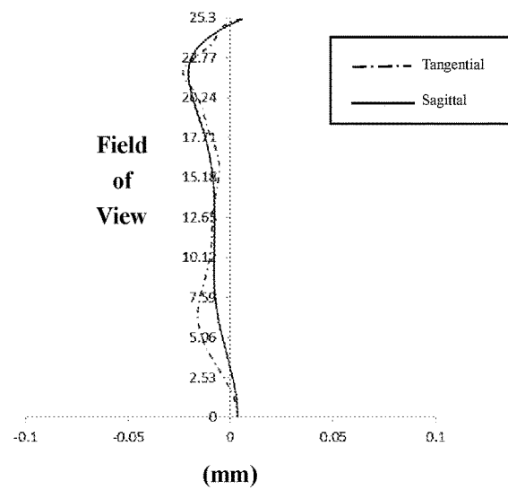
Astigmatism Curve
