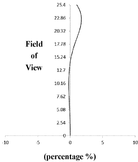
Distortion Curve
