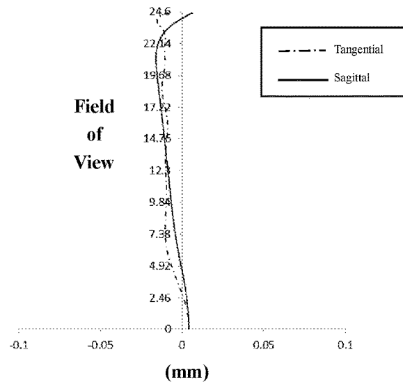
Astigmatism Curve
