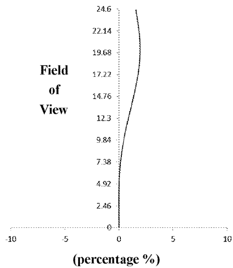
Distortion Curve
