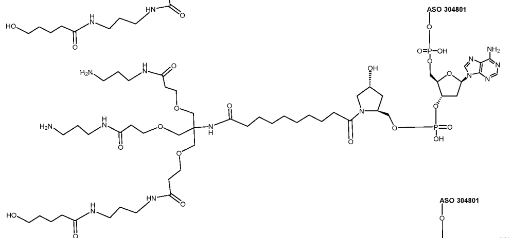
Metabolite 5
