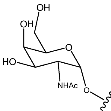
2-(Acetylamino)-2-deoxy-α-D-galactopyranose
