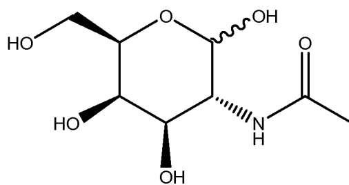
2-(Acetylamino)-2-deoxy-D-galactopyranose
