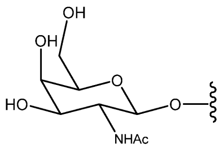
2-(Acetylamino)-2-deoxy-β-D-galactopyranose
