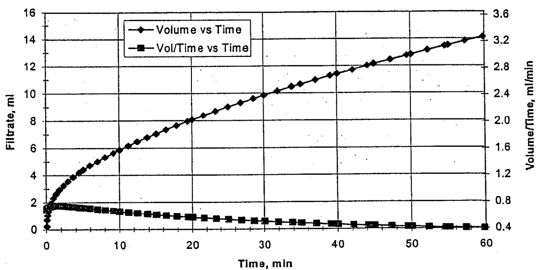
One - Hour Fann 90 Data for K-Citrate at 300°F
