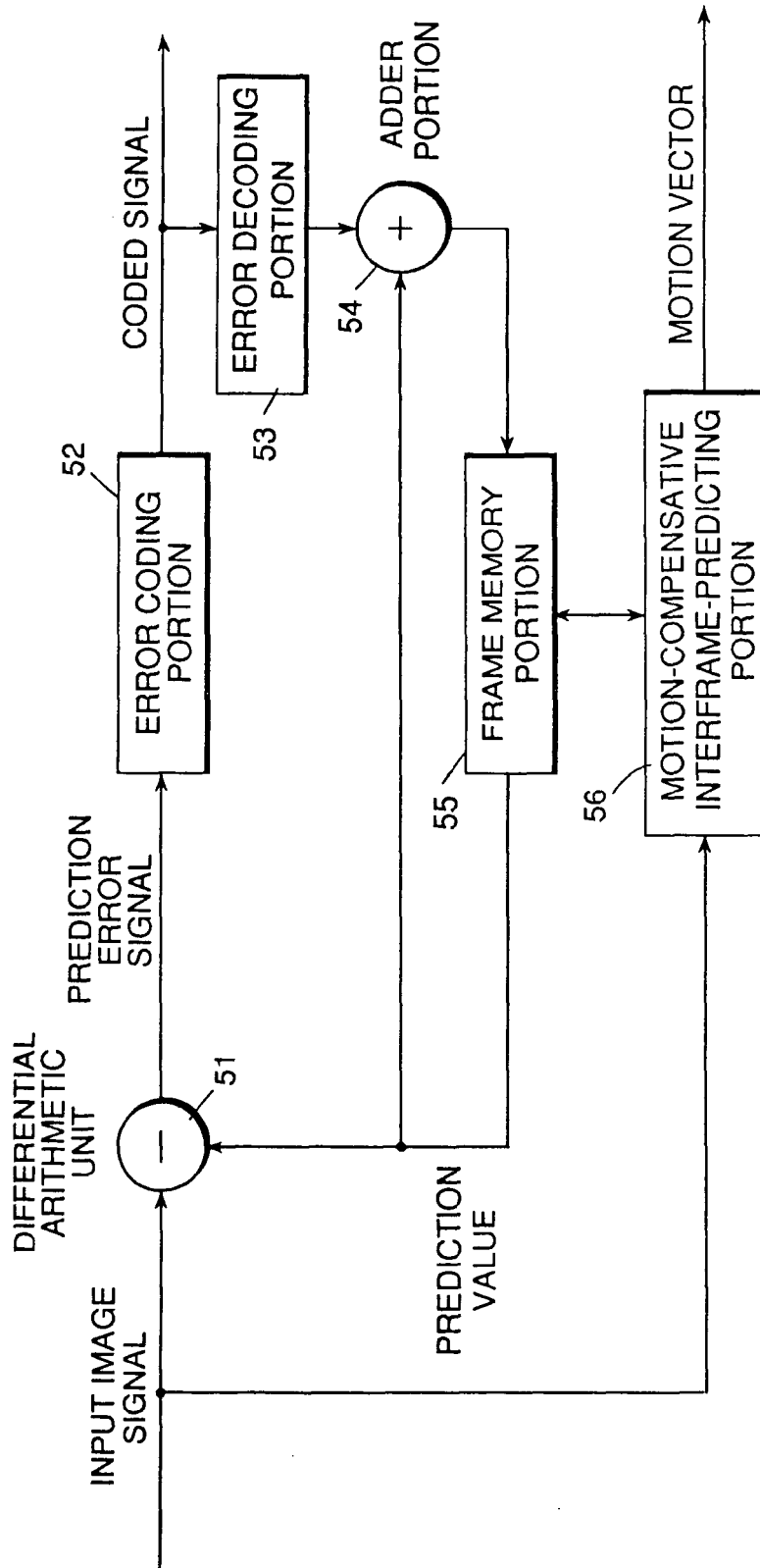
FIG.8 ( PRIOR ART )
