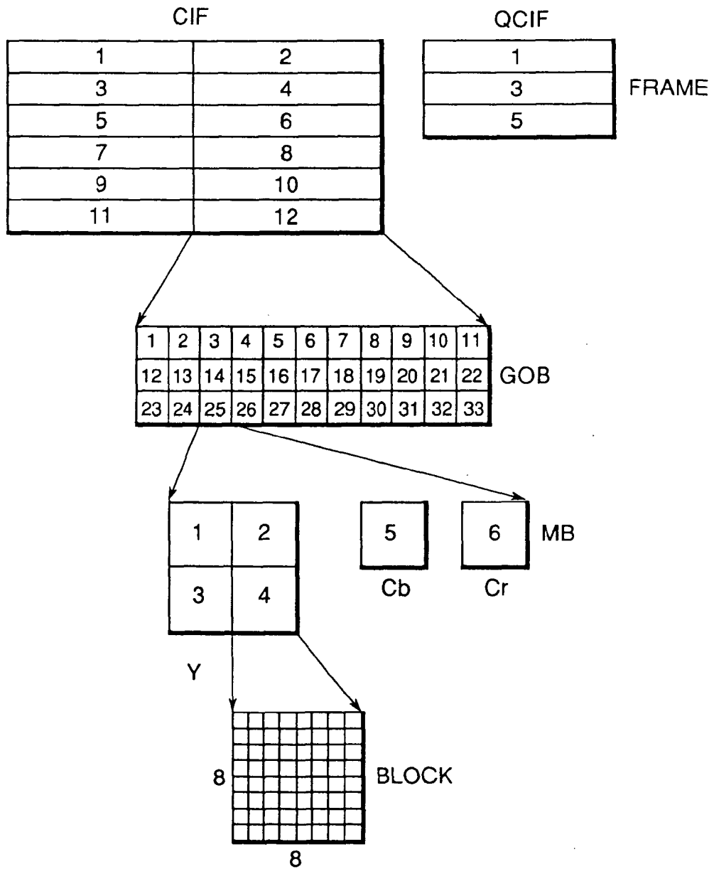
FIG.5 ( PRIOR ART )
