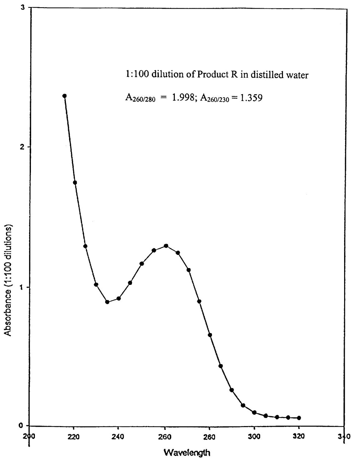
Figure 1. Ultraviolet Spectrum of Product R
