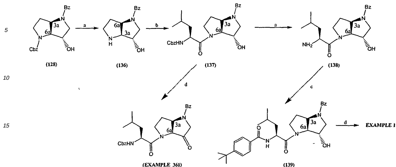
Scheme 27. (a) Pd-C / H 2 , ethanol / methanol. (b) leq Cbz-Leu-F, DMF, RT. (c) 1.05eq 4- tert -butylbenzoic acid, HBTU, HOBT, NMM, DMF, RT (d) Dess-Martin periodinane, DCM.
