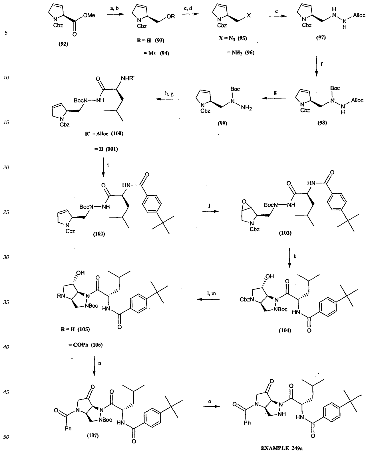
Scheme 23. (a) DIBAL-H, THF or \text{LiBH}_4 , MeOH, THF (b) Methanesulfonyl chloride, triethylamine, DCM (c) Sodium azide, DMF, 110^\circ\text{C} (d) \text{Ph}_3\text{P} / \text{H}_2\text{O} , 1,4-dioxane, 50^\circ\text{C} (e) 3-Phenylloxaziridine-2-carboxylic acid allyl ester, DCM (f) (\text{Boc})_2\text{O} , DCM, 60^\circ\text{C} (g) \text{Pd}(\text{PPh}_3)_4 , \text{PhSiH}_3 , DCM (h) Alloc-Leu-F, DMF (i) 4- tert -Butylbenzoic acid, HBTU, HOBT, NMM, DMF (j) m -Chloroperoxybenzoic acid, DCM. (k) Potassium carbonate, \text{CH}_3\text{CN} , 60^\circ\text{C} (l) Pd-C, \text{H}_2 , ethanol (m) (\text{PhCO})_2\text{O} , DMF (n) Dess-Martin periodinane, DCM (o) TFA, DCM
