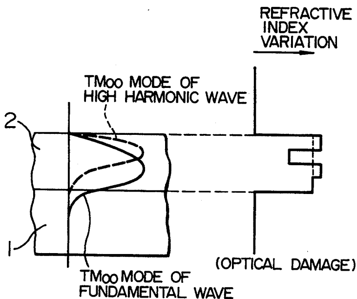
PRIOR ART FIG. 20b
