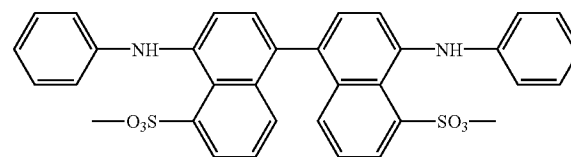
Structure of bis-ANS
