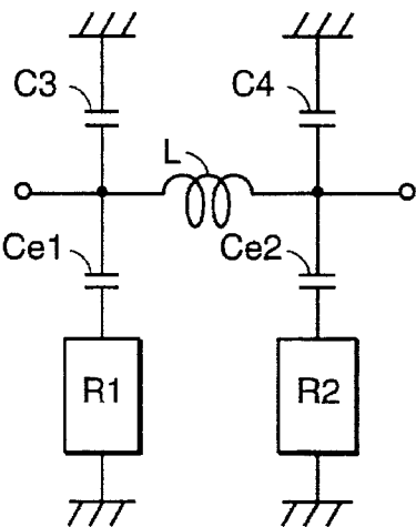
FIG._14 (PRIOR ART)
