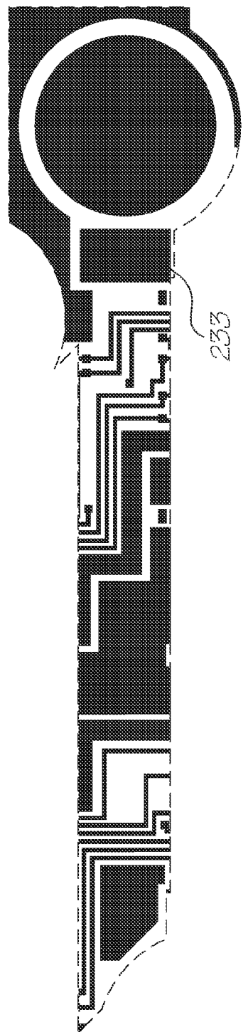
Metal 2 mask
