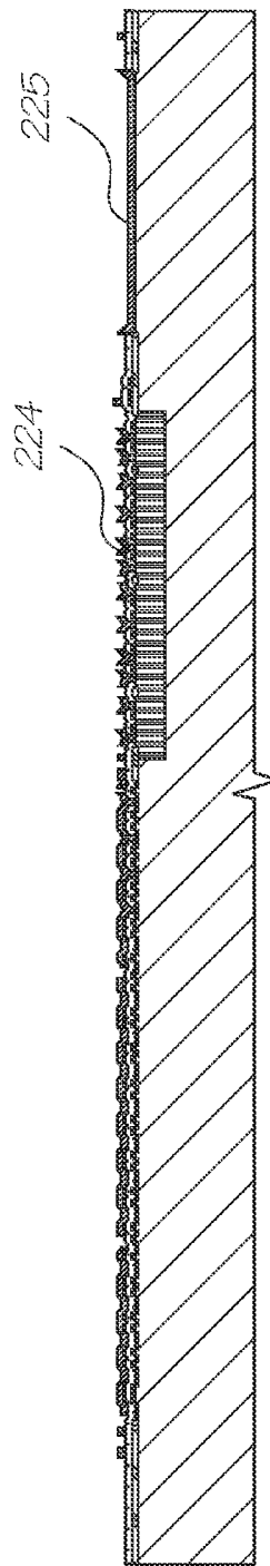
Deposit Metal 1
