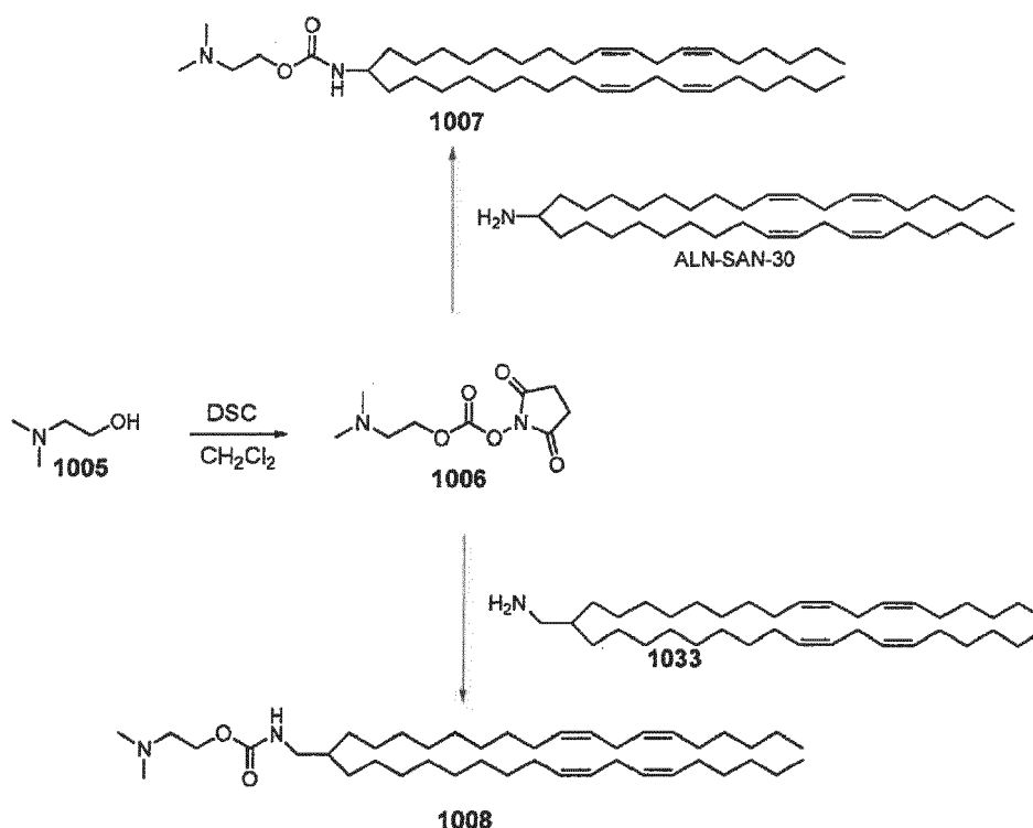
Scheme 3
