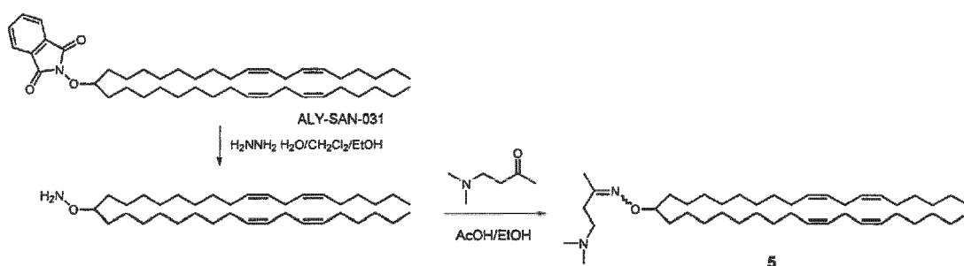
Compound 6
