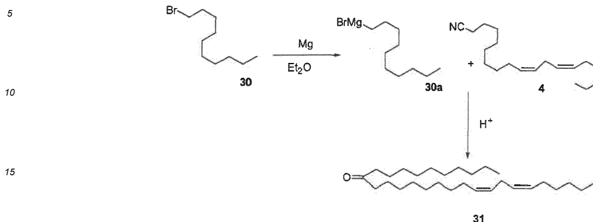
Scheme 5
