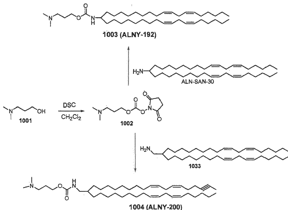
Scheme 2
