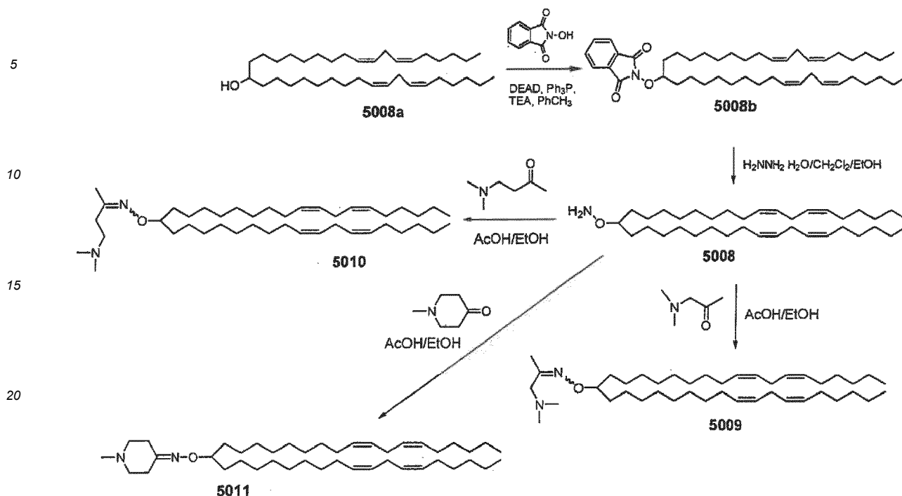
Scheme 2.
