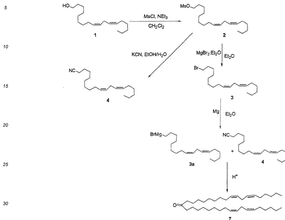
Scheme 1
