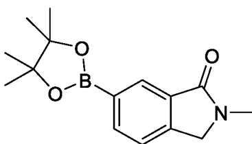
2-Methyl-6-(4,4,5,5-tetramethyl-1,3,2-dioxaborolan-2-yl)isoindolin-1-one
