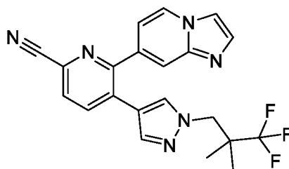
6-(imidazo[1,2-a]pyridin-7-yl)-5-(1-(3,3,3-trifluoro-2,2-dimethylpropyl)-1H-pyrazol-4-yl)picolinonitrile (Scheme 2)
