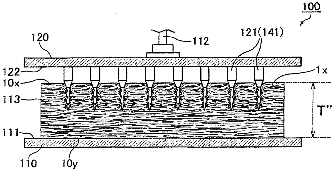
D-D line cross-sectional view
