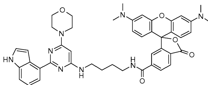
Isomer 1
