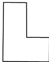
\partial M
