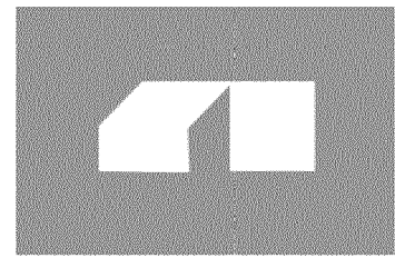
Int(Shape(M'))
