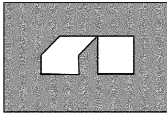
Shape(M')
