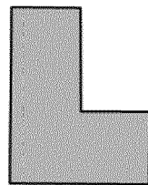
Shape(M)
