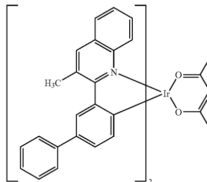
Ir(5-Ph-3'-Mepq) 2 (acac)
