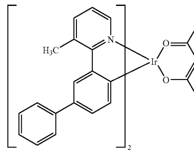
Ir(5-3'-Mepq) 2 (acac)
