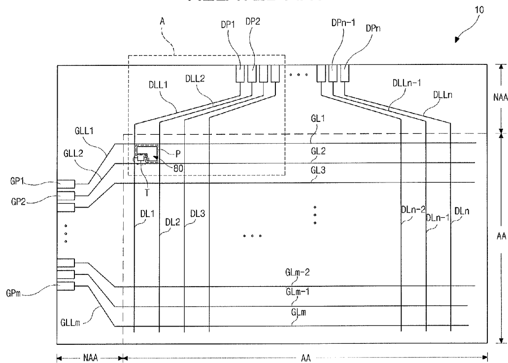
FIG. 1 RELATED ART
