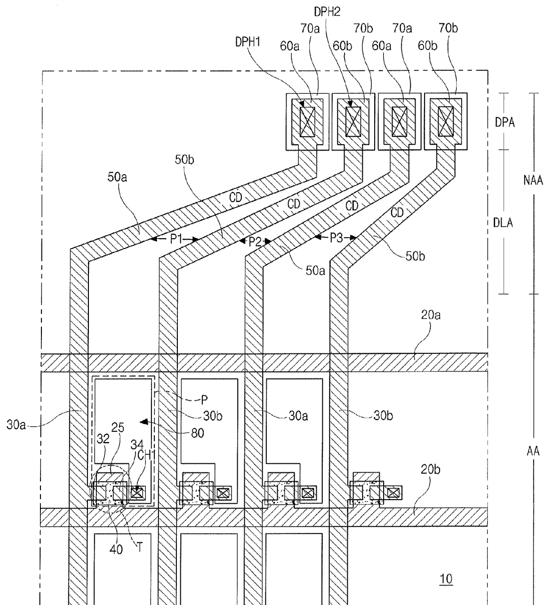
FIG. 2 RELATED ART
