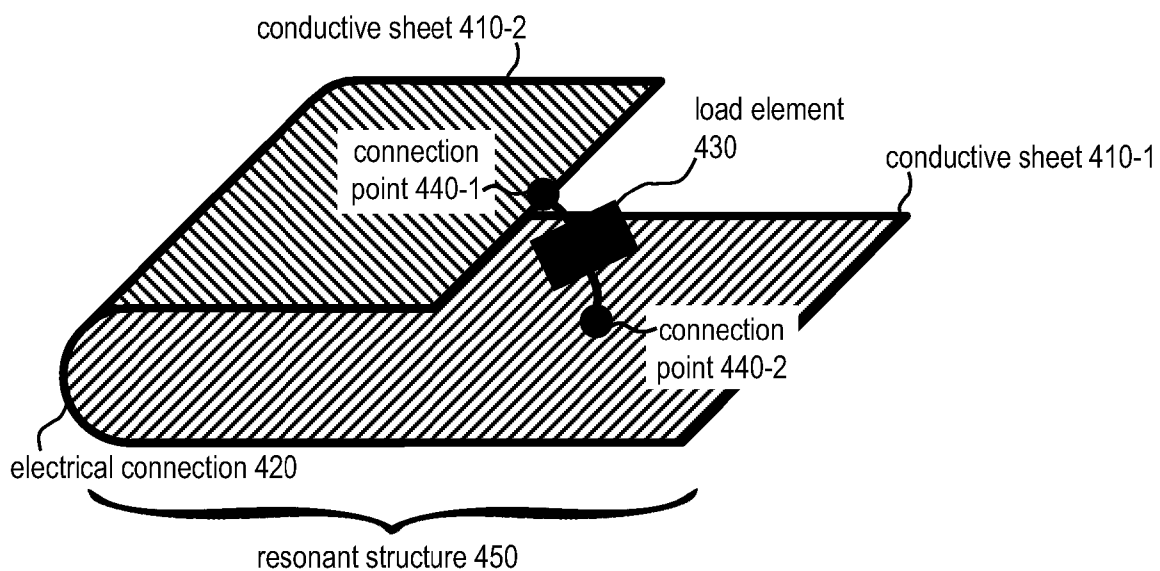
FIG. 4 PRIOR ART Single-cavity antenna with load element 400
