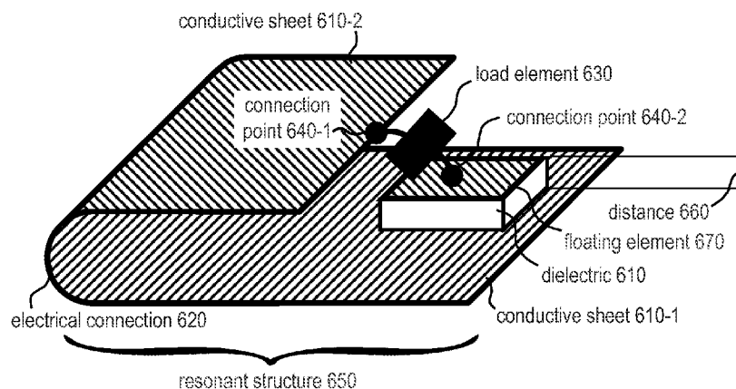
Single-cavity antenna with floating element and dielectric 600
